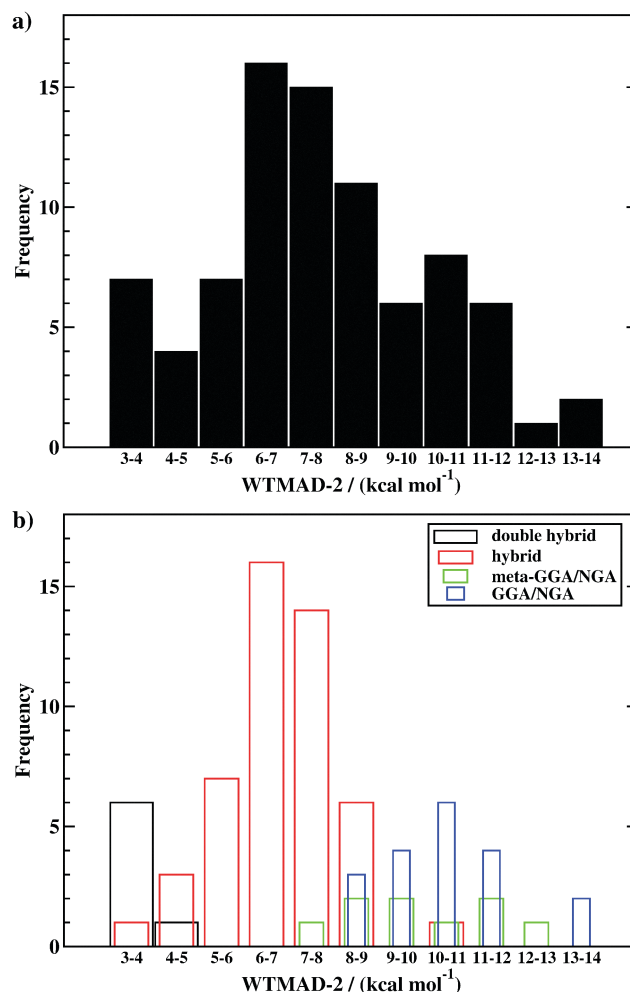
Fig. 7 Histograms ( 1 \text{ kcal mol}^{-1} bins) showing the WTMAD-2 distributions for all 83 dispersion-corrected DFAs (a) and for each rung of Jacob's Ladder (b).
