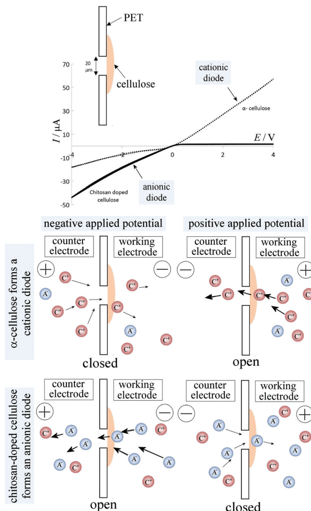
Fig. 5 Cyclic voltammograms (scan rate: 20 \text{mV s}^{-1} ) of \alpha -cellulose only films (dotted line) and chitosan-doped PET cellulose films (black solid line) on a 20 \mu\text{m} diameter microhole in a PET sheet in 50 mM NaCl on both sides of the membrane. The schematic drawing shows the four mechanistic cases of a cationic diode and an anionic diode under positive potential and negative potential polarisation, respectively.
