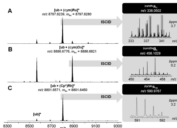
Fig. 2 Ultra-high resolution ESI-TOF mass spectra of 2:1 reaction mixtures containing 1a (A), 1b (B) or 1c (C) and after 24 h (left). ISCID top-down signals of the respective mono-adduct revealed Met1 as the primary metallation site (right).
