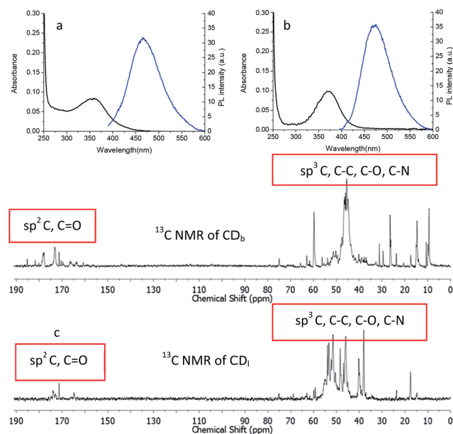
Fig. 3 UV-Vis absorbance and photo luminescent emission spectra (excited at 360 nm) of the carbon dots passivated with (a) branched PEI (CD b ) and (b) linear PEI (CD i ). (c) ^{13}C NMR spectrum of CD b and CD i .
