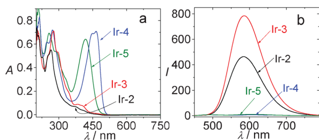
Fig. 19 (a) UV-vis absorption of Ir-2 , Ir-3 , Ir-4 and Ir-5 . In \text{CH}_3\text{CN} ( 1.0 \times 10^{-5} M; 20^\circ\text{C} ). (b) Emission spectra of the \text{Ir}^{\text{III}} complexes. Ir-2 : \lambda_{\text{ex}} = 386 nm, Ir-3 : \lambda_{\text{ex}} = 407 nm, Ir-4 : \lambda_{\text{ex}} = 462 nm, Ir-5 : \lambda_{\text{ex}} = 421 nm. In deaerated \text{CH}_3\text{CN} ( 1.0 \times 10^{-5} M; 20^\circ\text{C} ). Reproduced with permission from ref. 45b.
