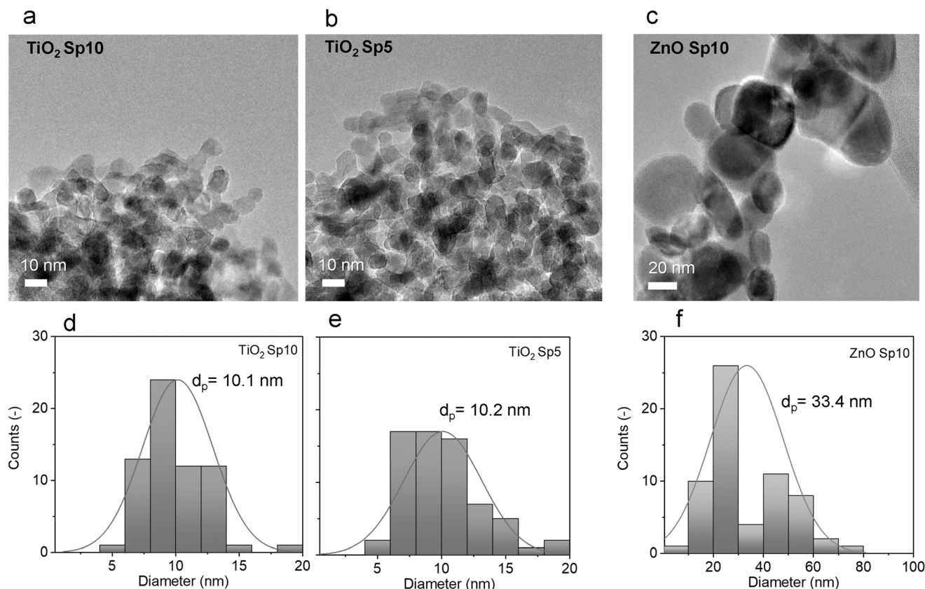
Fig. 5 TEM images of a) titanium dioxide (TiO 2 ) Sp10, b) TiO 2 Sp5, and c) zinc oxide (ZnO) Sp10 spark-ablated nanoparticles using 10 l min -1 (Sp10) and 5 l min -1 (Sp5) flow rates, for nanoparticle generation and deposition; d)–f) the corresponding particle size distributions.
