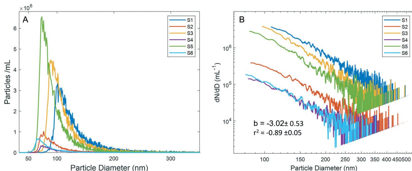
Fig. 2 A) Particle size distributions for ^{27}\text{Al} obtained by spICP-QMS. B) Reprocessed PSD data, with data normalized to number per nm ( \text{dN}/\text{dD} ) versus diameter and plotted in log space. The slope ( b ) and r^2 are an average of all samples; \pm 1 SD.
