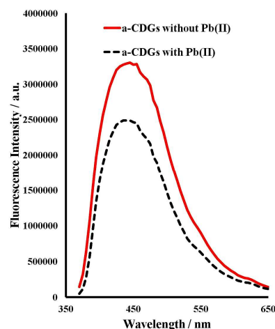
Figure 7. (a) Photoluminescent response to 10 \mu\text{g}\cdot\text{mL}^{-1} of \text{Pb}^{2+} to CD solutions, CD-containing hydrogels (CDGs) and CD solutions in the presence of dissolved gelator (1 \text{mg}\cdot\text{mL}^{-1} , \lambda_{\text{ex}} = 370 \text{ nm} ) and for 1 w.t. % CD-gels with 1a at the same CD concentration. (b) Fluorescence emission spectra for a -CD gel samples with and without \text{Pb}^{2+} (10 \mu\text{g}\cdot\text{mL}^{-1} ).
