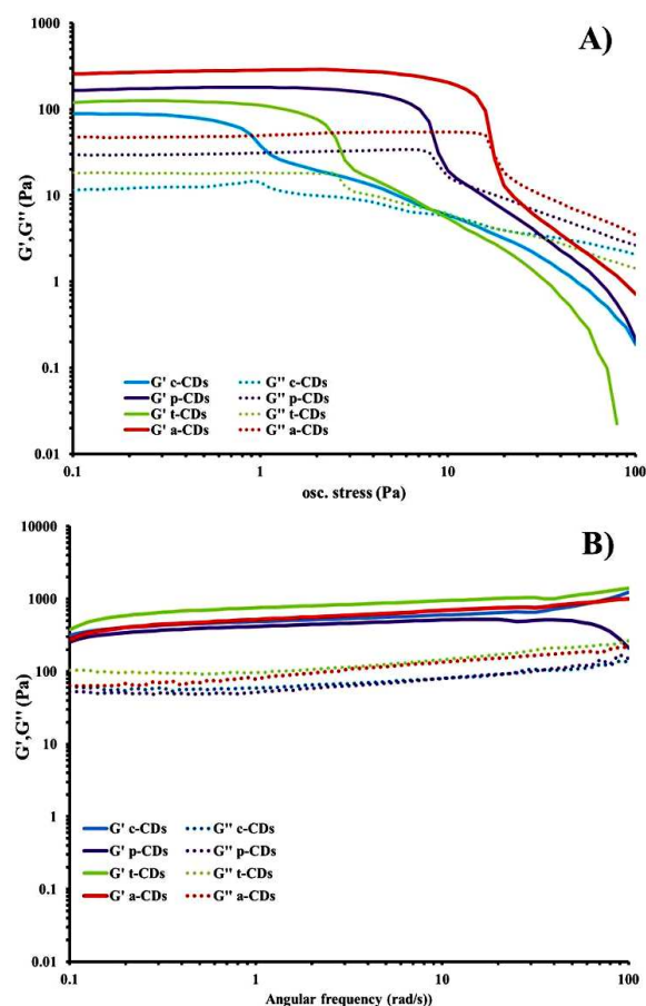
Figure 4. (a) Stress sweep and (b) frequency-sweep rheology of dilute ionic-liquid CD-Gel hybrid materials of composition 1 w.t. % 1a in 500 \mu\text{L} of CD solution at 1 \text{mg mL}^{-1} containing 2 % BMIM-BF 4
