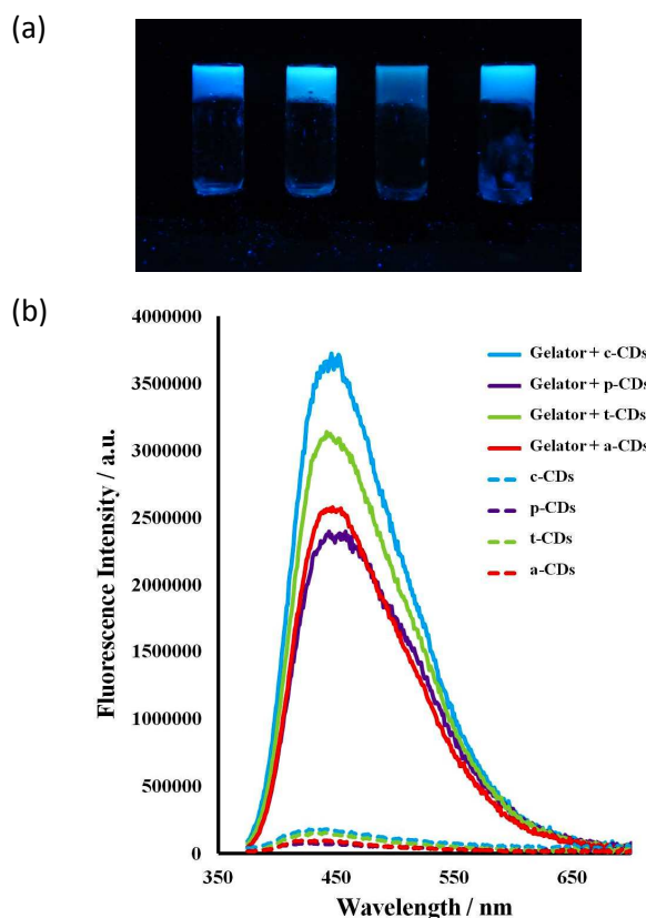
Figure 6. (a) a -, c -, p - and t -CD gels 1 w. t. % under 365 nm UV irradiation. (b) Fluorescence emission spectra of aqueous CD solutions (1 \text{mg mL}^{-1} , \lambda_{\text{ex}} = 365 nm for c -CDs and 370 nm for the others) and for 1 w.t. % CD-gels with 1a at the same CD concentration. Slits at 2 nm.
