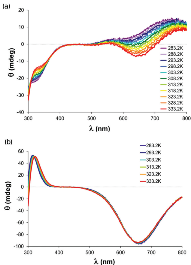
Fig. 4 Temperature dependent CD spectra recorded in the 300–800 nm wavelength range for equimolar systems of copper(II) and (a) His-Ala with the [\text{CuL}]^+ complex dominating at pH = 5.00, (b) Gly-Leu with the peptide-type [\text{CuLH}_{-1}] complex dominating at pH = 7.00 in the equilibrium system. The copper(II) ion concentration was \sim 5.0 \times 10^{-3} M in a cuvette with 1 cm optical path length.
