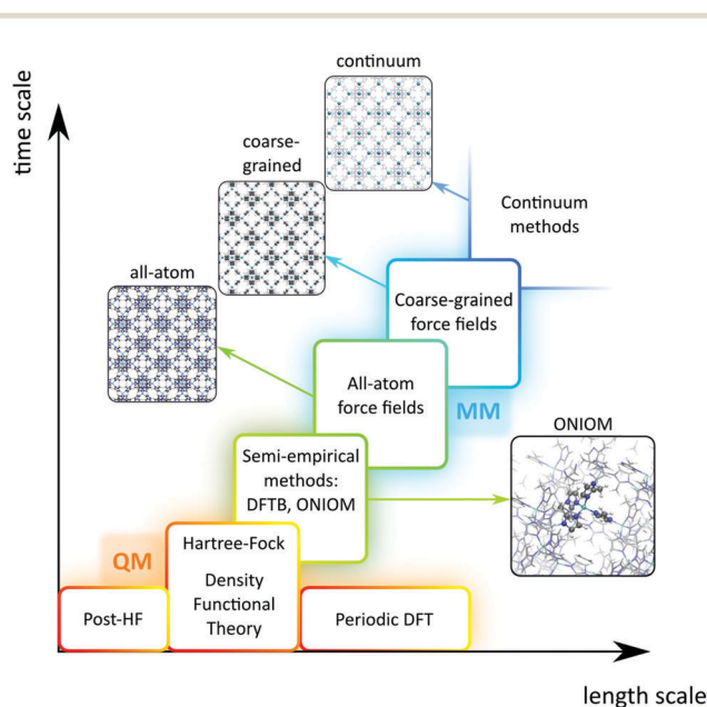
Fig. 9 Schematic overview of length and time scales of methods going from purely quantum mechanical (QM) based methods to force field (MM) and coarse-grained methods.
