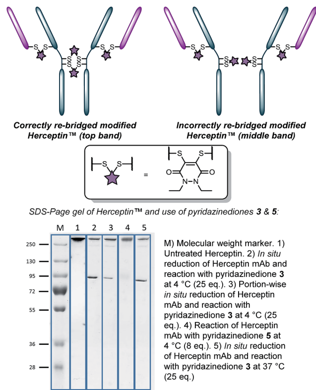
Fig. 2 Appraisal of the use of pyridazinediones 3 ( in situ 4 °C (pre-reduced, portion-wise reduction), 37 °C) and 5 for functional re-bridging of Herceptin TM .
