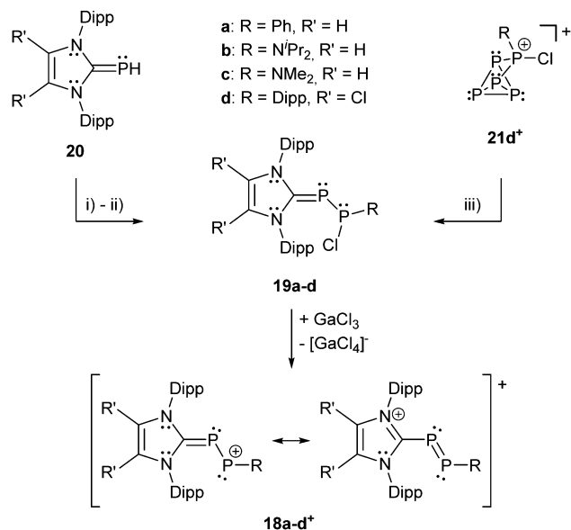
Scheme 7 Two different approaches for the synthesis of NHC stabilized chlorodiphosphanes 19a–d comprising bonding motif B . For 19a,b : (i) +R_2PCl_2 , +DABCO, -DABCO \cdot HCl ; for 19c : (ii) +2 PCl(NMe_2)_2 , +DABCO, -DABCO \cdot HCl , -P(NMe_2)_3 ; for 19d : (iii) +3 1,3-bis(2,6-diisopropylphenyl)-4,5-dichloro-imidazole-2-ylidene, -5^+ . Subsequent chloride abstraction yields polarized cationic diphosphenes 18a–d + . Only two resonance structures that indicate the polarization of 18a–d + are shown.
