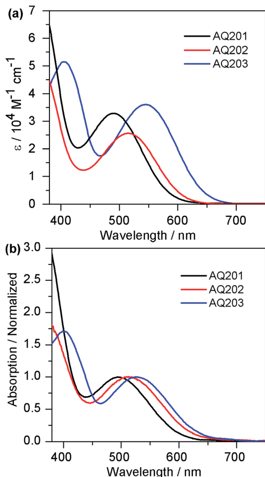
Fig. 1 (a) Absorption spectra of dyes AQ201, AQ202, and AQ203 in CH 2 Cl 2 ; (b) normalized absorption spectra of dyes AQ201, AQ202, and AQ203 on 4 μm TiO 2 films.
