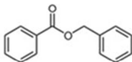
Benzyl benzoate
