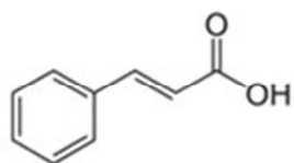
cinnamic acid
