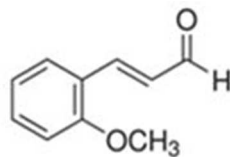
O-methoxy cinnamaldehyde
