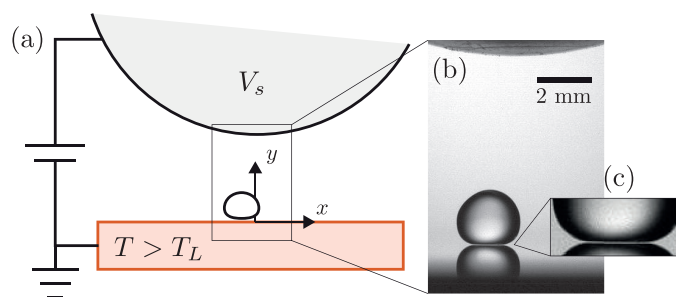
Fig. 1 (a) Schematic of the setup. A droplet hovering on a hot plate ( T > T_L ) is trapped under a spherical electrode set to a high voltage V_s between 2 and 5 kV. (b) Image captured by the high speed camera just after deposition. It shows a millimetric droplet of ethanol and its reflection in the polished aluminum plate. In the magnification of the contact region (c) the thin vapor gap, which insulates the drop from the hot surface is clearly visible.
