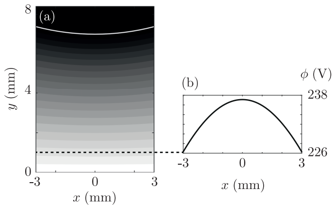
Fig. 9 (a) Electrical potential between a conducting sphere of V_s = 2\text{ kV} (black) and a grounded plate (white). (b) Horizontal slice through the field in (a) showing the weak trapping potential close to the plate.
