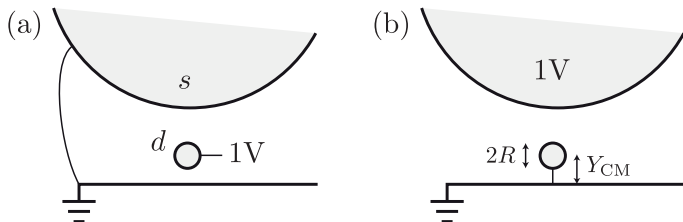
Fig. 4 Canonical electrostatic problems to calculate the capacitance coefficients in our experiment. The height Y_{CM} and radius R of the droplet are varied. From (a) we get c_{dd}(Y, R) = Q_d and c_{sd}(Y, R) = Q_s , and in (b) we have c_{ds}(Y, R) = Q_d and c_{ss}(Y, R) = Q_s .
