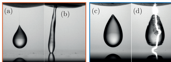
Fig. 8 Instabilities observed for (a-b) ethanol and (c-d) water droplets at voltage differences above 4 kV. In (a) the ethanol droplet developed a sharp cone from which small droplets are ejected. A few bounces later (b) it temporarily formed a vertical bridge between the top electrode and the hot bottom plate, still hovering on a vapor film. Also the water droplet (c) first developed a cone, but in this case (d) the electrical tension is released by a violent discharge that ruptures the drop.
