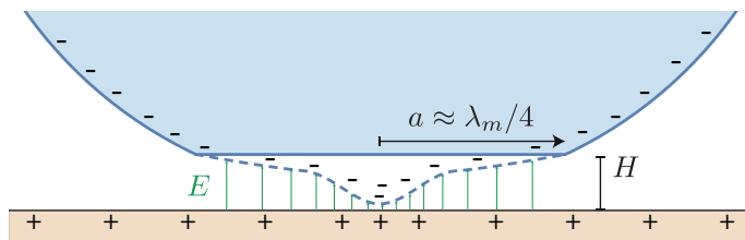
Fig. 5 Cartoon of the electro-capillary instability in the vapor gap that we speculate to be at the root of the observed discharge events.
