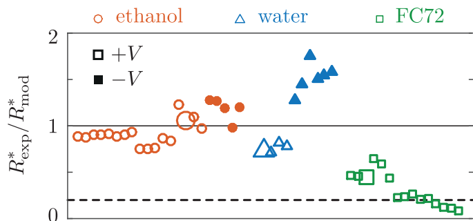
Fig. 6 Escape radius of the droplet (just before impact) in repeated experiments at various voltages ( \pm(2-5) \text{ kV} ) and temperatures ( 120-300^\circ \text{C} ), normalized by the predicted critical radius R^* given by equation (8). For the dashed line the low dielectric constant of FC72 was taken into account. The large symbols correspond to the representative cases shown in figure 3.
