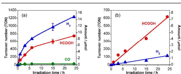
Fig. 2 Time courses of \text{HCOOH} (red), \text{H}_2 (blue) and \text{CO} (green) formation by visible-light ( \lambda > 400 nm) irradiation to \text{RuRu}/\text{Ag}/\text{TaON} (4 mg) in \text{EDTA}\cdot 2\text{Na} (10 mM) aqueous solution (4 mL) without (a) and with (b) \text{Na}_2\text{CO}_3 (0.1 M) under a \text{CO}_2 atmosphere.
