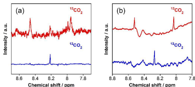
Fig. 7 1 H NMR spectra of reaction solutions (2 mL) containing RuRu/Ag-TaON (8 mg) in (a) H 2 O–MeOH (4:1 v/v) and (b) H 2 O–iPrOH (4:1 v/v) after a 48-h irradiation with visible light ( \lambda > 400 nm) under 13 CO 2 (red) and 12 CO 2 (blue) atmospheres.
