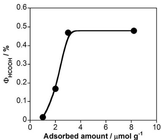
Fig. 5 Relationship between Φ HCOOH and loading amount of RuRu in the photocatalytic reaction using RuRu /Ag/TaON (30 mg) and EDTA-2Na (10 mM) in aqueous solution (10 mL) with 400-nm monochromatic light irradiation under a CO 2 atmosphere.
