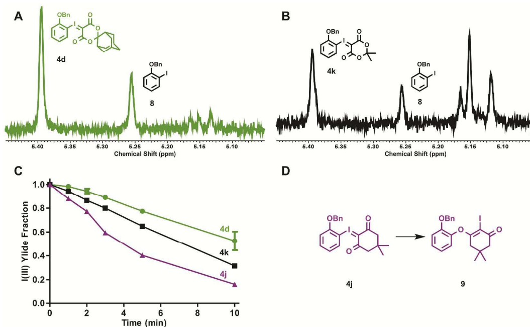
Fig. 6 Stability of electron rich iodonium ylides (SPIAd- 4d , Meldrum’s acid- 4k , and dimedone- 4j ) under reaction conditions in absence of [ 18 F]fluoride. Conditions: 3.5 μmol iodonium ylide in 0.7 mL DMF- d 7 (5 mM) + TEAB (4.8 mg/mL, 25 mM), heated to 120 °C ( n = 2)
