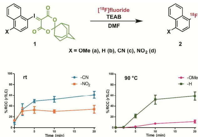
Fig. 3 Effect of substituent electronics on radiofluorination. n = 3 for each data point; see SI for detailed procedure; error bars represent SD.
