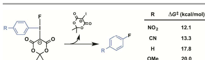
Fig. 4 Predicted influence of arene electronics on reductive elimination. PBE0-D3/aug-cc-pVTZ/SDB-aug-cc-pVTZ(l) single point, B3LYP/6-31G(d)/LANL2DZ(l)/PCM(DMF) geometry and vibrational correction.
