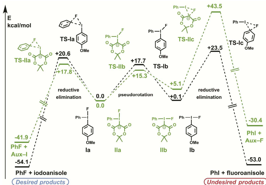
Fig. 2 Calculated reaction profiles for iodonium fluoride reductive elimination pathways. PBE0-D3/aug-cc-pVTZ/SDB-aug-cc-pVTZ(I) single point, B3LYP/6-31G(d)/LANL2DZ(I)/PCM(DMF) geometry and vibrational correction.
