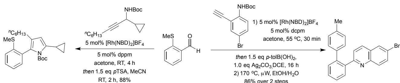
Scheme 10 Intermolecular hydroacylation routes to highly functionalised aza-heterocycles.
