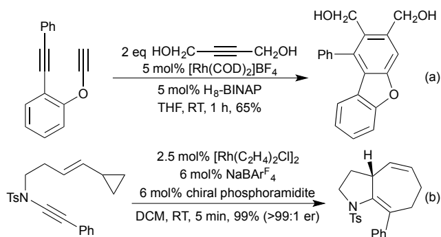
Scheme 5 Carbocycle formation, resulting in heterocyclic products.
