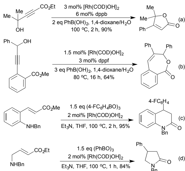
Scheme 16 Rh hydroarylation routes to diverse heterocycles.
