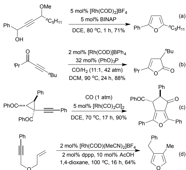
Scheme 4 Cycloisomerisation routes to oxygen containing heterocycles.
