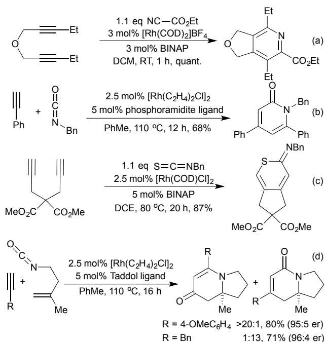
Scheme 6 [2+2+2] Cycloadditions to generate pyridine derivatives.
