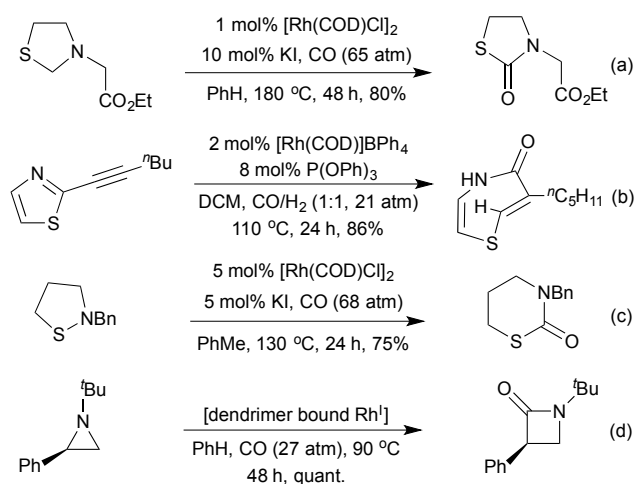
Scheme 24 Carbonylative ring-expansion reactions.
