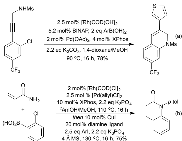
Scheme 17 Tandem Rh/Pd catalysis in heterocycle synthesis.
