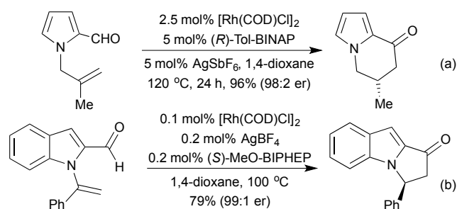
Scheme 13 Intramolecular hydroacylation on indole/pyrrole backbones.
