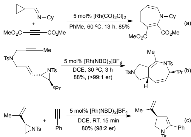
Scheme 8 aza-[5+2] and [3+2] cycloadditions to generate azaheterocycles
