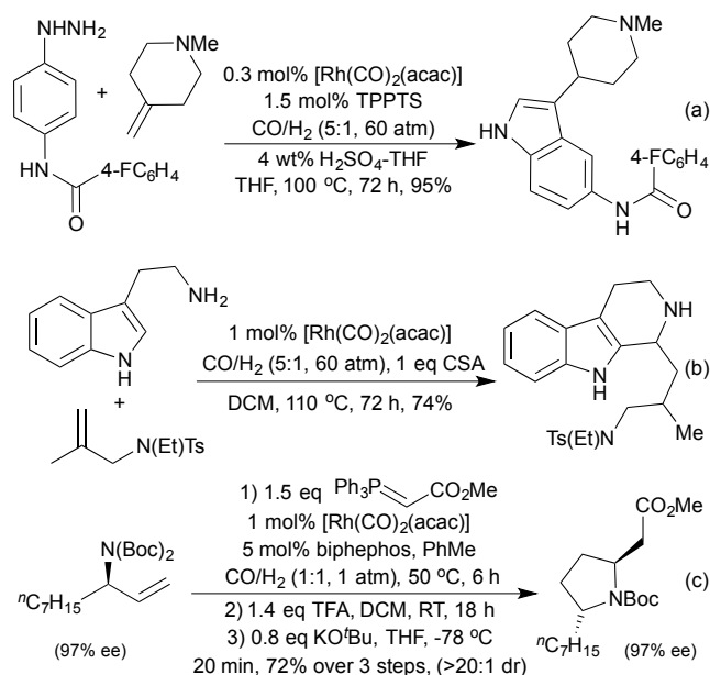
Scheme 21 Tandem hydroformylation/heterocyclisation reactions.
