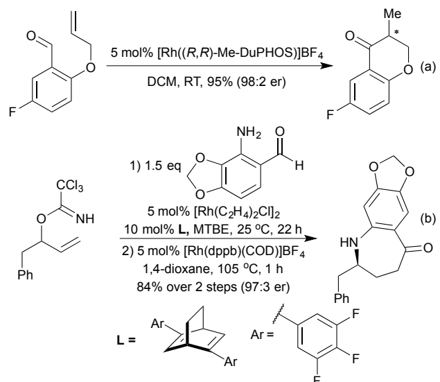
Scheme 12 Intramolecular alkene hydroacylation towards enantioenriched medium-ring heterocycles.
