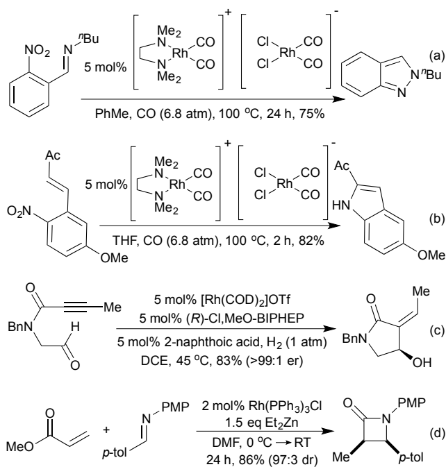
Scheme 25 Reductive cyclisation approaches to N -heterocycles.
