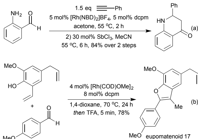
Scheme 11 Hydroacylation-based tether-incorporating heterocycle syntheses.
