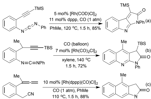
Scheme 9 [2+2+1] Pauson-Khand cycloaddition approaches to heterocycles.
