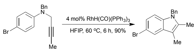
Scheme 3 Cascade [3,3]-sigmatropic rearrangement/hydroamination indole synthesis.
