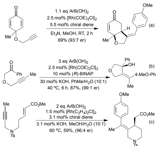
Scheme 19 Enantioselective cascade routes to saturated heterocycles
