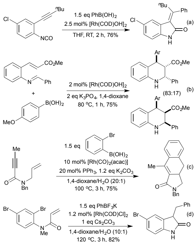
Scheme 18 Rh hydroarylation initiated domino reactions
