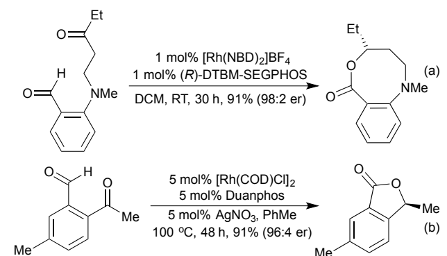
Scheme 14 Intramolecular ketone hydroacylation based lactone syntheses.
