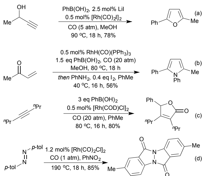
Scheme 23 Carbonylative 3-component couplings to form 5-membered heterocycles.
