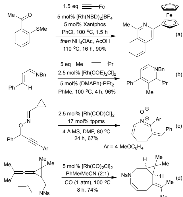
Scheme 26 Miscellaneous Rh(I) catalysed heterocycle syntheses.
