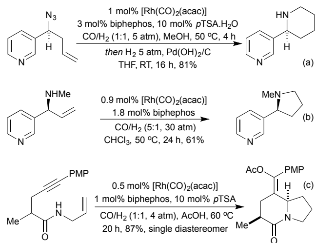
Scheme 22 Tandem hydroformylation reactions in alkaloid synthesis.
