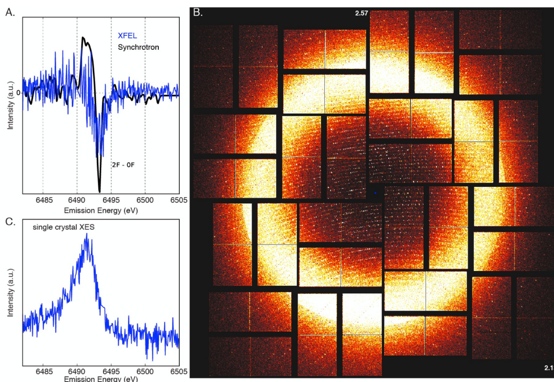
Figure 4: A. Overlay of the 2F-dark Mn K\beta_{1,3} XES difference spectra using an XFEL (blue) and a synchrotron (black). B. fs diffraction pattern of a PS II crystal in the 2 flash state recorded at room temperature, resolution in the corners is 2.13 Å and at the edges 2.57 Å, diffraction spots are visible beyond 2.3 Å resolution. C. Mn K\beta_{1,3} XES from PS II crystals in the 2F state. The spectrum was collected from an experimental run in which 1466 crystal hits were identified in the diffraction detector.
