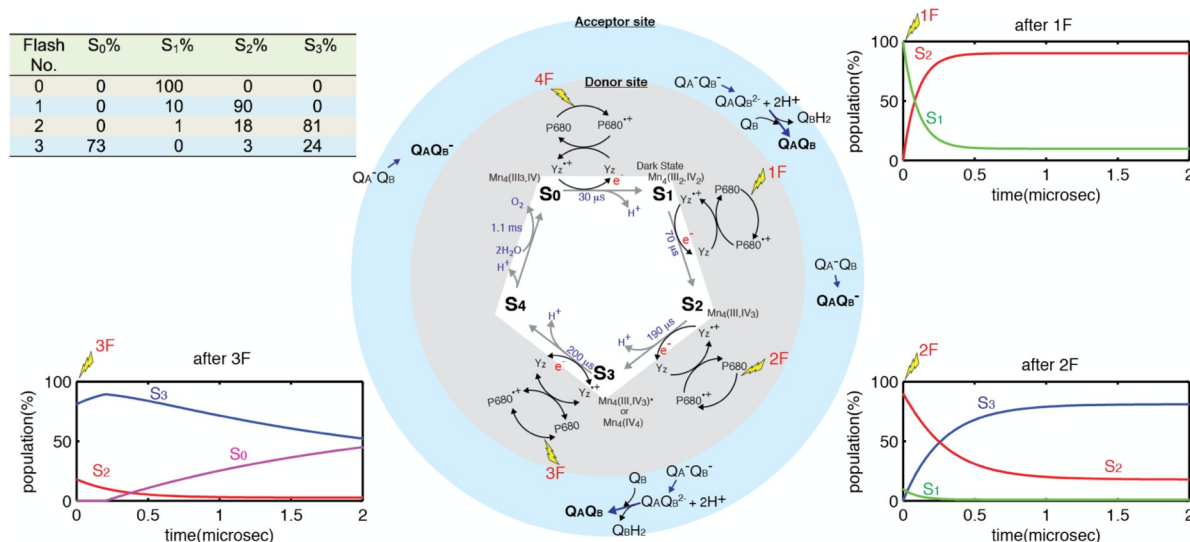
Figure 3: Center: The Kok S-state cycle for water oxidation by PSII. Gray - donor side: Each of the four photons absorbed by the PS II P680 reaction center, oxidizes the tyrosine Y_Z intermediate, which in turn oxidizes the Mn_4CaO_5 complex. Blue - acceptor side: Q_A and Q_B are reduced on the acceptor side. Left Top: A best case steady state S-state population as a function of laser-flash illuminations. 10% miss hit is assumed. Insets: The evolution of the populations of the S-states as a function of time are shown after 0 flashes (0F), 1 flash (1F) and 2 flashes (2F). 21-23
