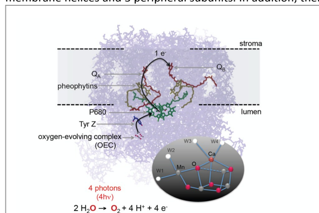
Figure 1: The electron transfer chain of Photosystem II. The inset shows the structure of the water oxidizing Mn 4 CaO 5 catalyst. 1
