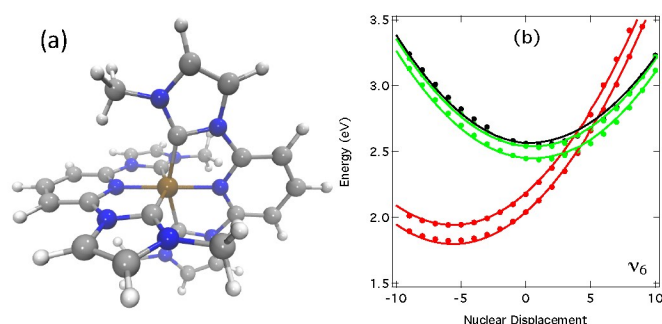
Fig. 1 (a) Molecular structure of [\text{Fe}(\text{bmip})_2]^{2+} . (b) Cut through the spin-free potential energy curves along v_6 , the most important for the excited state dynamics of [\text{Fe}(\text{bmip})_2]^{2+} . The dots are derived from the quantum chemistry calculations. The lines correspond to their fit from which the expansion coefficients of the diabatic Vibronic Coupling Hamiltonian are determined. Colour code is as follows: ^1\text{MLCT} : black, ^3\text{MLCT} : green and ^3\text{MC} : red.
