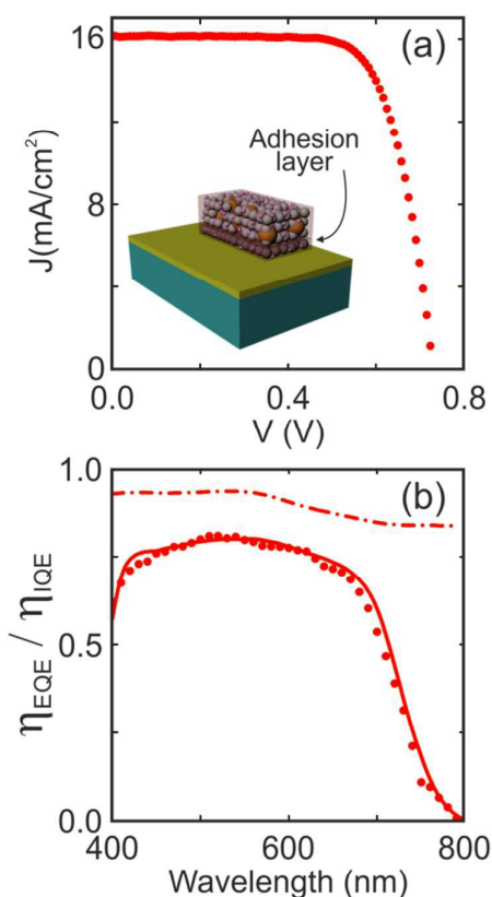
Figure 4. (a) Experimental J-V curve for a plastic cell with a total structured electrode thickness of (11.80 \pm 0.50) microns consisting of a first (2.65 \pm 0.15) micron adhesion layer without scatterers, and a second layer on top with 30% of nanoparticles of radius 160 nm. The schematics in the inset represent the considered electrode. (b) Experimental (symbols) and theoretical (solid lines) \eta_{EQE}(\lambda) spectra for the same system as that in panel (a). The effective electron diffusion length estimated from the fitting is L_e = 16 microns. Corresponding calculated \eta_{IQE}(\lambda) curves are displayed with dashed lines.
