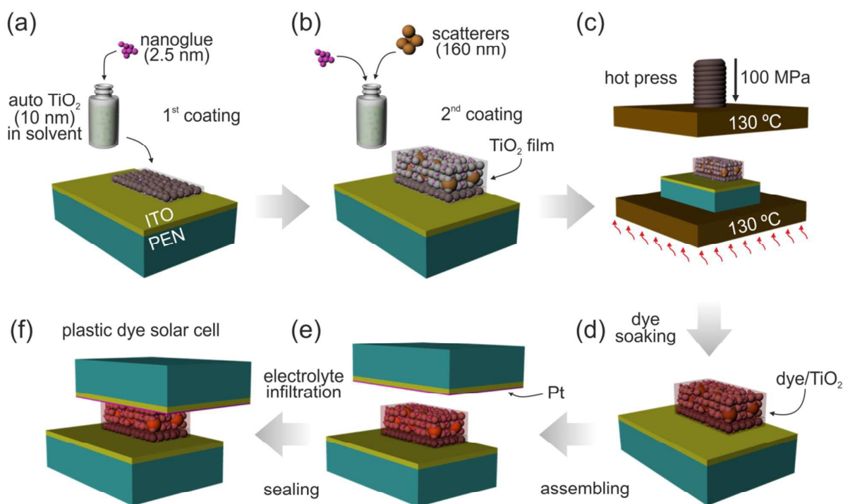
Figure 1. Schematic illustration of the final fabrication process of a plastic dye solar cell on flexible ITO/PEN substrate containing the necessary optimization steps. (a) A thin adhesion layer was coated by doctor blade method with 3M tape as a spacer from an organic binder free paste which was prepared by dispersing 2.5 nm radius nanoglue nanoparticles (NPs) with 10 nm radius \text{TiO}_2 NPs into the mixture solvent of EtOH and tert-butanol. (b) Main \text{TiO}_2 layer was coated with same method but with a 160 nm radius scattering NPs added paste. (c) Hot pressing, that is, physically pressing at 100 MPa simultaneously with heating at 130 °C to synergistically enhance the interconnection of \text{TiO}_2 NPs. (d) Dye soaking of \text{TiO}_2 film. (e) Electrolyte infiltration, and assembling dye sensitized \text{TiO}_2 film with a thermoplastic surlyn and a counter electrode composing of catalytic Pt layer on ITO/PEN substrate. (f) Hot sealing of electrodes by thermoplastic surlyn for a plastic dye solar cell.
