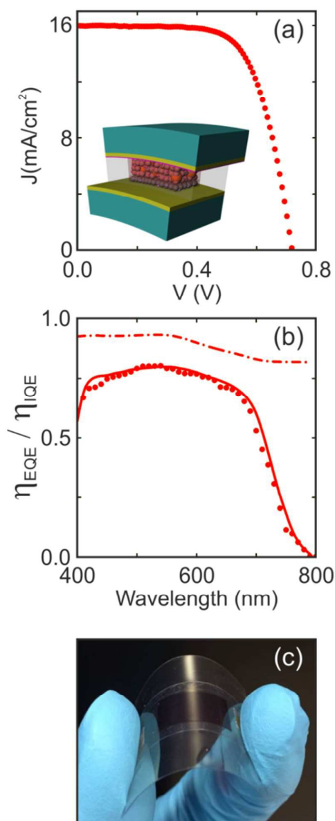
Figure 5. (a) Experimental J-V curve for a flexible cell with a total structured electrode thickness of (11.80 \pm 0.50) microns consisting on a first (2.65 \pm 0.15) microns layer without scatterers, and a second layer on top with 30% of light scatterers ( r = 160 nm). (b) Experimental (symbols) and theoretical (solid lines) \eta_{EQE}(\lambda) spectra for the same system as that considered in panel (a). The effective electron diffusion length estimated from the fitting is L_e = 16 microns. Corresponding calculated \eta_{IQE}(\lambda) curves are displayed with dashed lines. (c) Image of the fabricated flexible dye solar cell.
