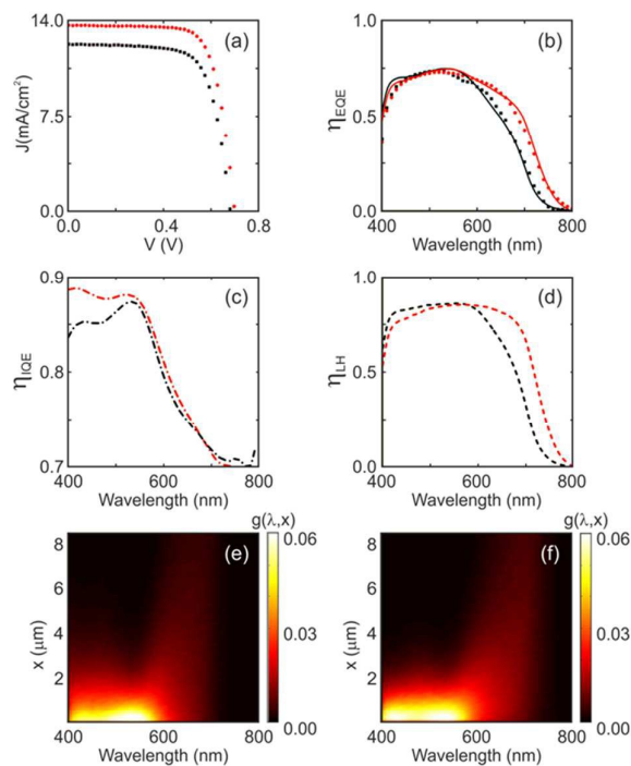
Figure 2. (a) Experimental J-V curves of plastic cells. Square black symbols correspond to an (8.60 \pm 0.05) microns electrode without scatterers, and circular red ones to an electrode of the same thickness with 30% of titania particles of radius 160 nm. (b) Experimental (symbols) and theoretical (solid lines) \eta_{EQE}(\lambda) spectra for the same systems as in panel (a). The “effective” electron diffusion length is taken to be L_e = 8 microns. (c) Corresponding calculated \eta_{IQE}(\lambda) (or equivalently \eta_{col}(\lambda) ) curves and (d) \eta_{LH}(\lambda) (or absorptance) spectra. (e) and (f) electron generation functions, or spectral absorption profiles g(\lambda, x) of each photoelectrode as a function of x and \lambda for a (e) reference cell without scatterers and (f) a DSC with 30% of light scatterers ( r = 160 nm).
