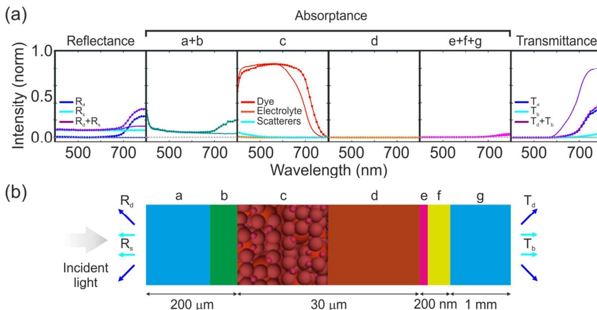
Figure 3. (a) Theoretical results of reflectance (left panel), absorbance (intermediate panels) and transmittance (right panel) for the same systems as those considered in Figure 2. Lines correspond to a reference cell without scatterers, and symbols with lines to a cell with 30% scatterers ( r = 160 nm). The cell is illuminated from the PEN substrate. Dashed grey line accounts for 0 reflectance, absorbance or transmittance. Diffuse and specular reflectance are labeled by R_d(\lambda) and R_s(\lambda) , respectively, and diffuse and ballistic transmittance by T_d(\lambda) and T_b(\lambda) , respectively. Each absorbance panel correspond to each element comprising the cell: [a+b] PEN and ITO substrate, [c] electrode (distinguishing each component, i.e., dye molecules, electrolyte and \text{TiO}_2 scatterers in the case of the electrode containing light scatterers), [d] electrolyte, and [e+f+g] counter electrode (platinized FTO and glass). (b) Schematic of the multilayer DSC containing light scatterers, displaying corresponding slab thicknesses.
