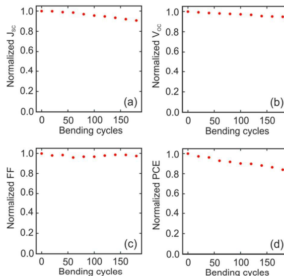
Figure 6. Normalized photonic characterization ( J_{sc} in panel (a), V_{oc} in panel (b), FF in panel (c) and PCE in panel (d)) of the optimized flexible cell in Figure 5 as a function of bending cycles with radius 15 mm.
