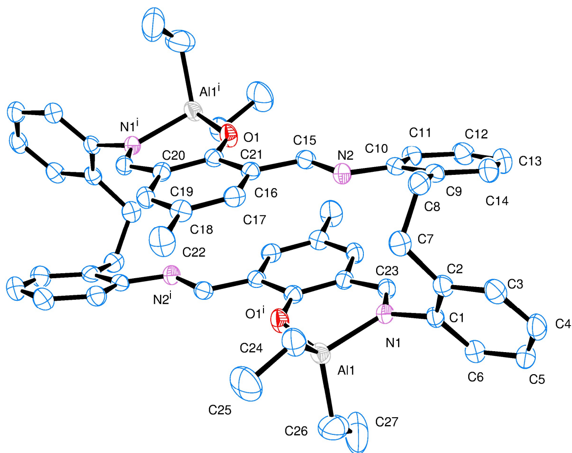
Figure 4. Molecular structure of [(\text{AlEt}_2)_2\text{L}^4] ( 8 ), with atoms drawn as 50 % probability ellipsoids. Symmetry operator used to generate the second half of the molecule: i = 1-x, -y, 1-z . Hydrogen atoms and MeCN of crystallisation have been omitted for clarity. Selected bond lengths (Å) and angles (°):
