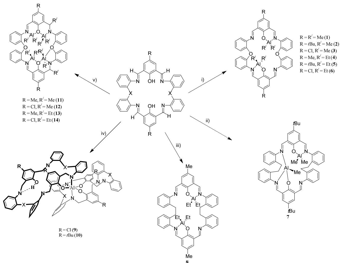
Chart 1. Synthesis of aluminium complexes 1 - 14 prepared herein. Reagents and conditions: i) 2R'_3\text{Al} , hexane, \Delta , 12 h; ii) 2\text{Me}_3\text{Al} , toluene, \Delta , 12 h; iii) 2\text{Et}_3\text{Al} , toluene, \Delta , 12 h; iv) \frac{1}{2}\text{Et}_3\text{Al} , hexane, \Delta , 12 h; v) 4R'_3\text{Al} , hexane, \Delta , 12 h.
