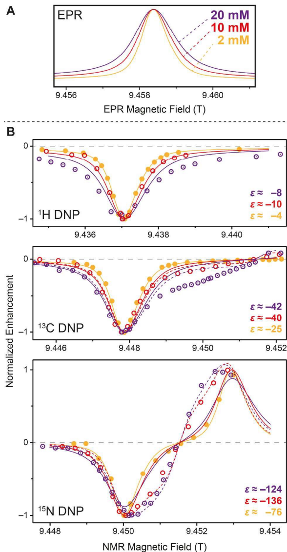
Figure 7. (A) EPR spectra of 2 mM (orange), 10 mM (red), and 20 mM (purple) Gd-DOTA at 263 GHz. Curves were obtained by simulating experimental cw (field-modulated) EPR spectra using Easyspin 95 in order to avoid artifacts by integration. (B) Normalized DNP enhancement of ^1\text{H} , ^{13}\text{C} , and ^{15}\text{N} at 263 GHz at 2 mM (filled circles), 10 mM (open circles), and 20 mM (dotted open circles). Solid lines represent SE simulations according to eq. (1); dashed lines CE simulations according to eq. (2). Enhancement factors given are taken at field of maximum magnitude enhancement.
