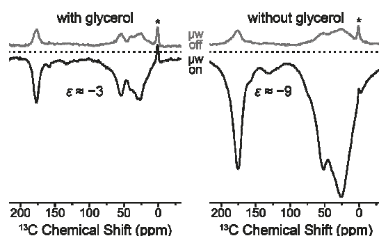
Figure 9. Direct DNP enhancement of uniformly [ 13 C, 15 N]-labeled ubiquitin mutant F4C with and without added glycerol using site-directed spin labeling with Gd-DOTA-M tags at 9.4 T. The field was optimized for Gd 3+ 13 C SE resulting in negative signal enhancement. Read-out was performed via Bloch decay with 4 s polarization delay. Asterisks mark signals from silicone plugs.
