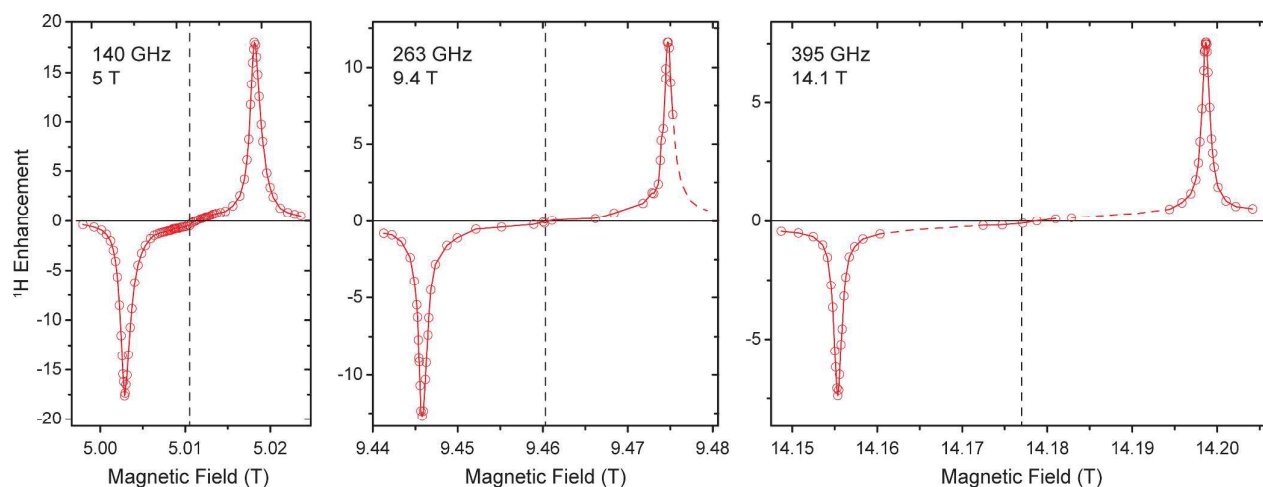
Figure 6. Comparison between field-dependent ^1\text{H} DNP profiles of 10 mM Gd-DOTA in \text{D}_8\text{-glycerol}/\text{D}_2\text{O}/\text{H}_2\text{O} (60:30:10 vol.-%) at 140, 263, and 395 GHz \mu\text{w} frequency. The EPR resonance fields are marked with dashed lines.
