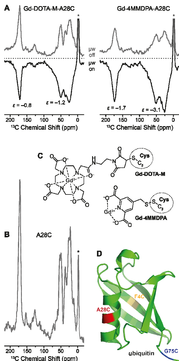
Figure 8. (A) Direct ^{13}\text{C} DNP enhancement of uniformly ^{13}\text{C} , ^{15}\text{N} -labeled ubiquitin mutant A28C using site-directed spin labeling with Gd-DOTA-M and Gd-4MMDPA tags at 9.4 T. The field was optimized for \text{Gd}^{3+} ^{13}\text{C} SE resulting in negative signal enhancement. Read-out was performed via Bloch decay with 6 and 2.3 s polarization delay, respectively. (B) ^{13}\text{C} MAS spectrum of A28C ubiquitin (without attached spin label), read-out via Bloch decay and 16 s polarization delay. Asterisks mark signals from silicone plugs. (C) Chemical structures of Gd-4MMDPA and Gd-DOTA-M spin labels connected to cysteine residues. (D) Ribbon structure of ubiquitin (PDB ID 1UBQ) with F4C, A28C, and G75C single-site mutations marked in yellow, red, and blue, respectively.
