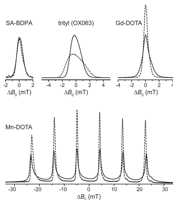
Figure 2. 140 GHz (solid lines) and 275 GHz (dashed lines) field-swept, echo-detected EPR spectra of SA-BDPA, trityl, Gd-DOTA, and Mn-DOTA demonstrating the narrowing of the high-spin CT at higher field. All spectra (except Mn-DOTA) were normalized to equal amplitude at 140 GHz. All 275 GHz spectra were scaled so that the respective integrals at the two frequencies are equal. Field offset in abscissa is given w.r.t. to the resonance field observed for the isotropic g value.
