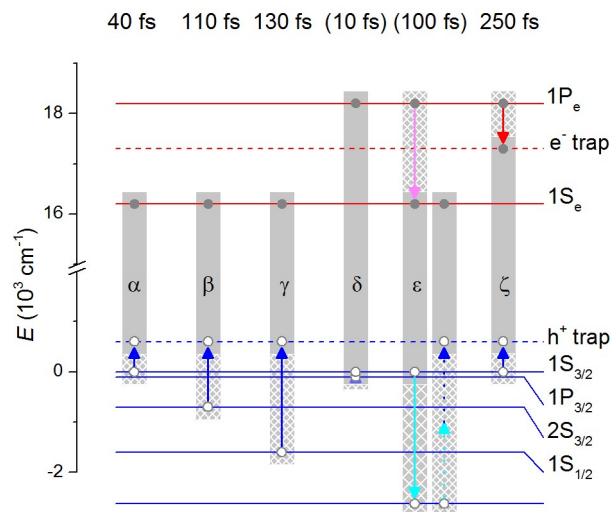
Fig. 5 Relaxation (magenta for electrons, cyan for holes) and trapping (red and blue) pathways (arrows). At the top are the obtained or estimated (in parenthesis) time constants of the processes. \alpha , \beta , and \gamma are the trapping pathways of |X_1\rangle , |X_2\rangle , and |X_3\rangle , respectively. \delta , \epsilon , \zeta are the pathways from the |X_4\rangle state, assuming the |1P_{3/2}\rangle hole relaxes to |1S_{3/2}\rangle as the first step ( \delta ). From there, either \epsilon or \zeta is followed. \epsilon consists of several substeps: first Auger relaxation, with the hole going into an unspecified state, followed by hole relaxation and trapping from this state, which was not studied in detail in our work. The first step of \epsilon is prevented by either electron trapping from |1P_e\rangle or hole trapping from |1S_{3/2}\rangle which happen in parallel rather than simultaneously and together form pathway \zeta . If the \delta step does not happen, \epsilon and \zeta will have the hole in |1P_{3/2}\rangle instead of |1S_{3/2}\rangle . The light grey rectangles mark the excitons before (solid and densely patterned) and after (solid and sparsely patterned) each step.
