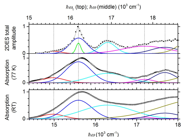
Fig. 2 To identify the electronic states of the QDs, we fit a slice of the 2D spectrum along with absorption spectra. All panels show fits of data (black squares) as a sum (gray line) of Gaussians (colored lines), average energies marked by vertical dashed lines) corresponding to specific states. Values were normalized to the maximum. Top panel: 2D total signal amplitude along a cut at \hbar\omega_3 = 16200 \text{ cm}^{-1} and T = 10 \text{ ps} , divided by the laser spectrum. Middle panel: Absorption spectrum at 77 K, smoothed and with a linear background subtracted. Bottom panel: As middle panel, but at room temperature. The spectrum is shifted by 610 \text{ cm}^{-1} to lower energies compared to at 77 K, and the x -axis is shifted correspondingly to align the peaks. For peak positions, see Figure 4.
