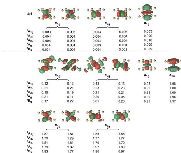
Figure 3. Orbitals in the (10,15) active space and their occupations in the various states of [Mn@Si_{12}]^+ (B3LYP geometry). Orbitals were generated for the ^1A_{1g} state using an isosurface value of 0.04.
