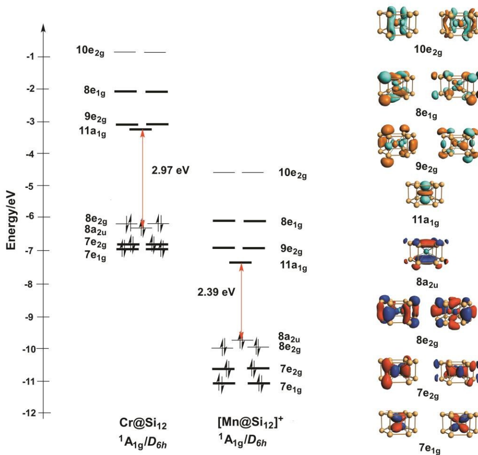
Figure 1. Comparison of the Kohn-Sham MO diagrams for \text{Cr@Si}_{12} and [\text{Mn@Si}_{12}]^+ (B3LYP functional, isosurface value = 0.04 ( e/\text{au}^3 ) 1/2 ). Orbitals with substantial metal 3d character are shown in bold.
