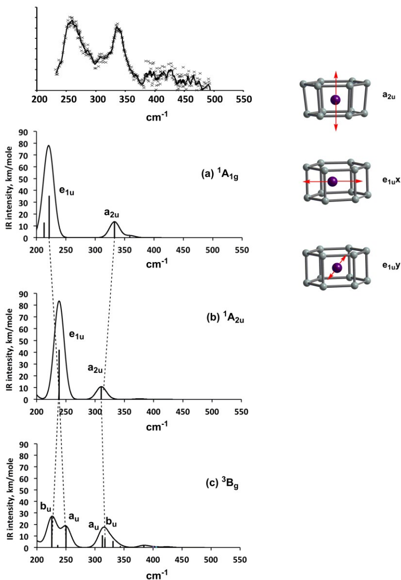
Figure 4. Experimental Infra-red multi-photon dissociation (IRMPD) spectrum of [\text{Mn@Si}_{12}]^{\dagger} and simulated vibrational spectra of the {}^1\text{A}_{1g} , {}^1\text{A}_{2u} and {}^3\text{B}_g states.
