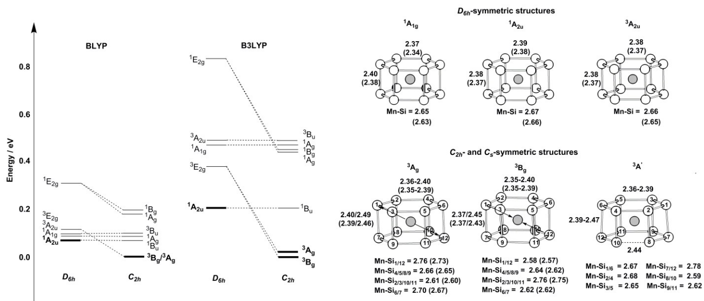
Figure 2. The energy landscape for [\text{Mn@Si}_{12}]^+ obtained with both BLYP and B3LYP functionals and the corresponding optimised structural parameters (bond lengths obtained with B3LYP are shown in parentheses).
