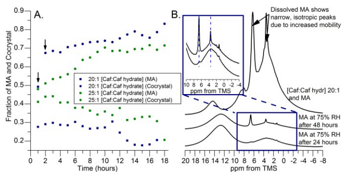
Figure 5. A. Kinetics of Caf:MA co-crystallisation process for mixtures of Caf:Caf hydrate with 20:1 and 25:1 [Caf:Caf hydrate] molar ratio. B. 1 H solid-state NMR spectra of MA after 24 and 48 hours storage at 75 % RH and [Caf:Caf hydr] 20:1 mixture with MA.
