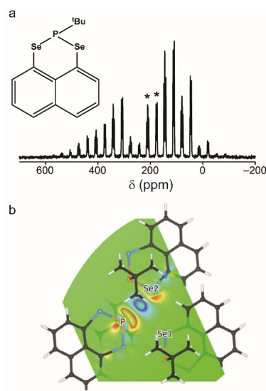
Figure 3. (a) ^{77}\text{Se} (9.4 T, 5 kHz MAS) NMR spectrum of 1 , with isotropic centreband multiplets denoted *. (b) CDD plot of the ^{77}\text{Se} - ^{31}\text{P} through-space J coupling in 1 at the PBE/USP (non-relativistic) level. Reprinted with permission from Ref. 57 Copyright 2015 American Chemical Society.
