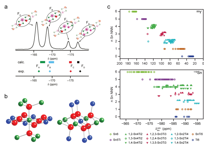
Figure 8. (a) ^{19}\text{F} MAS NMR spectra of (54%) fluorinated clinohumite ( 4\text{Mg}_2\text{SiO}_4\cdot\text{Mg}(\text{OH},\text{F})_2 ), with calculated chemical shifts for model structures with varying F substitution shown. Reprinted with permission from Ref. 47 Copyright 2010 American Chemical Society. (b) Local arrangement of atoms around the A (occupied by Y) and B (occupied by Sn or Ti) sites in a pyrochlore structure. (c) Plots showing the calculated ^{89}\text{Y} and ^{119}\text{Sn} isotropic chemical shifts as a function of the number of Sn NNN. Reprinted with permission from Ref. 53 Copyright 2009 American Chemical Society. Reproduced (in part) from Ref. 131 with permission of the PCCP Owner Societies.
