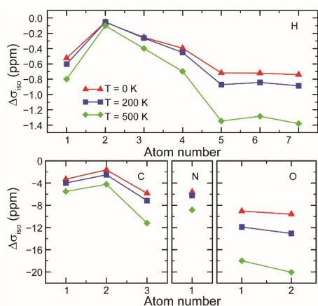
Figure 6. Change from static DFT ( \Delta\sigma_{\text{iso}}^{\text{calc}} = 0 ppm) in GIPAW isotropic shielding parameters of L-alanine with temperature corrections at 0, 200 and 500 K. Reprinted with permission from Ref. 109. Copyright 2014, AIP Publishing LLC.
