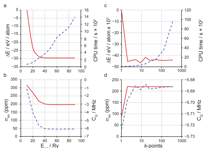
Figure 2. Plots demonstrating convergence of (a, c) \Delta E and CPU time and (b, d) \sigma_{iso} and C_0 against (a, b) E_{cut} and (c, d) number of k -points. In each case the red line corresponds to the left vertical axis and the dashed blue line to the right vertical axis.
