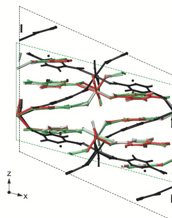
Figure 4. Overlay of the XRD structure of MIL-53(Sc) (green) and those optimised under PBE (black), PBE-D2 (grey) and PBE-TS (red).
