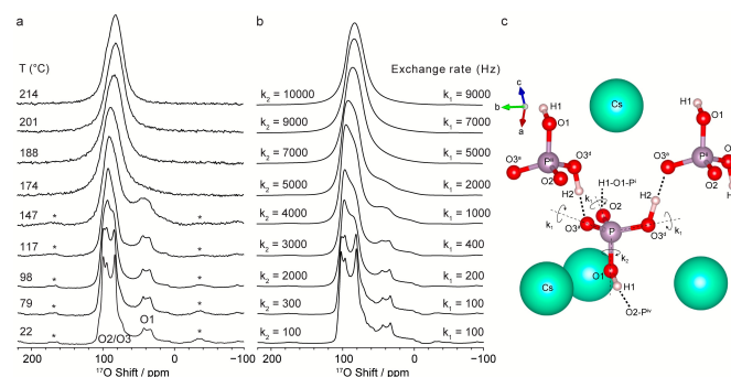
Figure 7. (a) 17 O (16.4 T) variable-temperature MAS NMR spectrum of CsH 2 PO 4 and (b) simulated 17 O lineshapes assuming exchange rates for rotations of k_1 and k_2 . (c) Structure around a phosphate ion showing bond rotations considered. Reproduced from Ref. 122.
