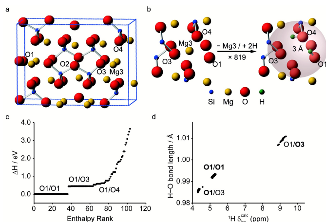
Figure 5. (a) View of the unit cell of \beta - \text{Mg}_2\text{SiO}_4 with (b) the AIRSS protocol used to produce 819 structures. (c) Enthalpy ranking of 103 AIRSS-generated structures chosen for more accurate DFT optimisation and NMR calculations (labels give the two sites of protonation). (d) Plot of H–O bond length against calculated ^1\text{H} \delta_{\text{iso}}^{\text{calc}} for low-enthalpy structures; bold text signifies the protonation site leading to the labelled data points). Reproduced (in part) from Ref. 103 with permission of the PCCP Owner Societies.
