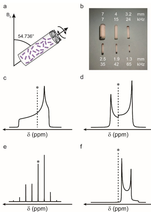
Figure 1. (a) Schematic showing the MAS rotor oriented at the magic angle with respect to the external magnetic field, B_0 . (b) Rotors used in MAS NMR experiments, showing outer diameters and maximum MAS rates. Schematic NMR lineshapes simulated under (c, d) static and (e, f) MAS conditions, for a (c, e) spin I = 1/2 and (d, f) spin I = 3/2 nucleus (central transition only). * denotes \delta_{iso} .
