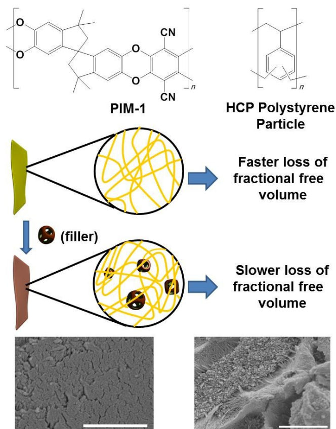
Figure 1. (Top) Molecular structure of PIM-1 and the hypercrosslinked polymer used as the filler. (Middle) Schematic illustration of effect of filler on overall performance of MMMs. SEM images of (bottom left) pristine PIM-1 and (bottom right) MMM with 16.67 wt% filler. Scale 1 μm.
