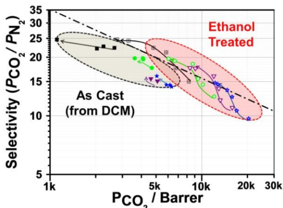
Figure 4. The single gas CO 2 permeability and ideal CO 2 /N 2 selectivity of PIM-1 based MMMs plotted against Robeson's 2008 Upper Bound. The filled squares and squares with the cross represent pure PIM-1 films. The filled shapes represent as cast, the open symbols the analogous films after ethanol treatment. The circles are for a filler content of 5.7 wt%, blue triangles for 16.7 wt% and green triangles for 21.3 wt% (As-cast data: 0→45→60→150 days; ethanol treated data: 0→15→30→45→90→150 days). Arrows indicate aging direction.
