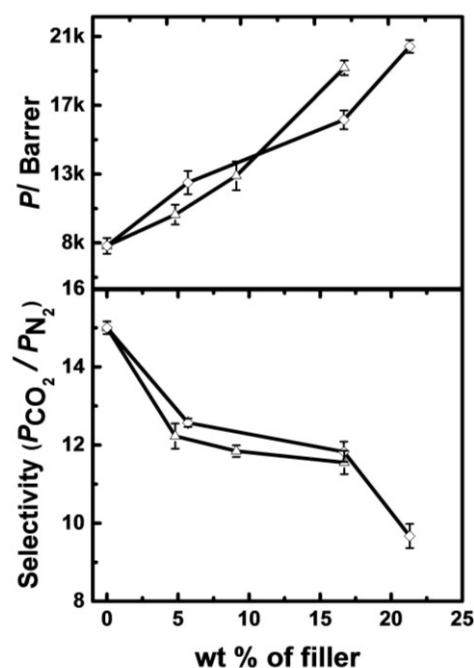
Figure 2. Dependence of permeability coefficient of CO 2 (top), and ideal selectivity relative to N 2 (bottom). (-o-): cast from DCM followed by ethanol treatment; (-Δ-): cast from chloroform followed by ethanol treatment. All data are shown for non-aged membranes.
