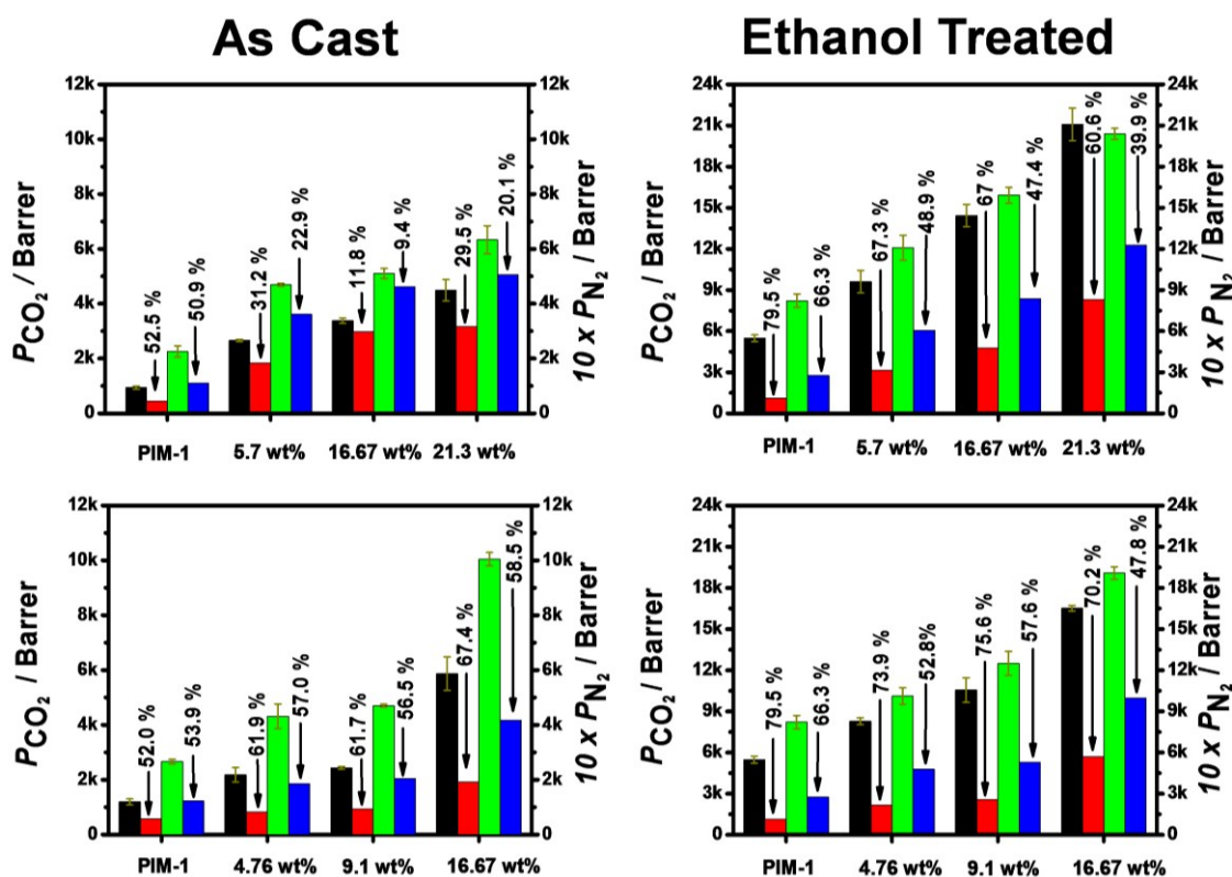
Figure 3. Permeability and aging characteristic of MMMs with HCP polystyrene as filler Top: cast from DCM and subsequent treatment by ethanol bottom: cast from chloroform and subsequent treatment by ethanol Colour code: (■) N_2 permeability on first day; (■) N_2 permeability on 150 th day; (■) CO_2 permeability on first day, (■) CO_2 permeability on 150 th day.
