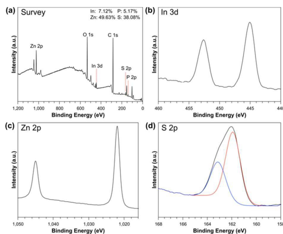
Figure 4. XPS representing the (a) Survey spectra of InP/ZnS NCs, (b) high resolution of In 3d, (c) Zn 2p and (d) S 2p spectra.
