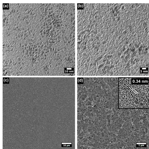
Figure 3. (a) TEM image of InP/ZnS NCs, (b) HRTEM of InP/ZnS NCs, (c) SEM showing overview of SWCNT photocathodes, (d) magnified SEM showing the network of SWCNTs. The inset shows the lattice fringes of the SWCNTs as measured with TEM.
