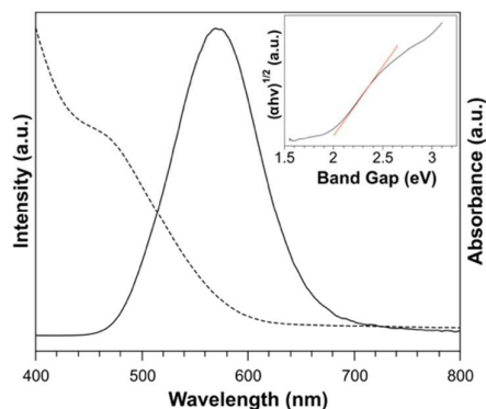
Figure 2. Absorbance (dashed line) and emission (solid line) spectra for InP/ZnS NCs. The inset shows a Tauc plot absorption spectrum for band gap estimation.
