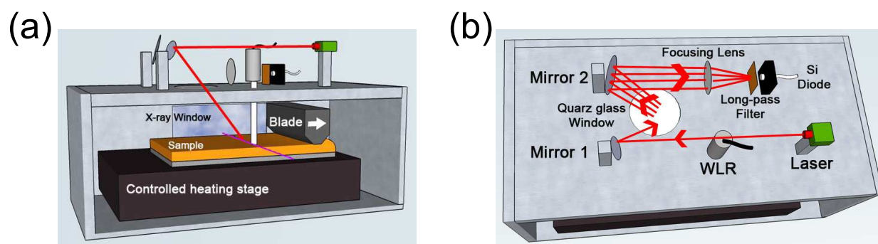
Fig. 1 Schematic illustration of the experimental chamber for in situ measurements of thin film drying from the side (a) and above (b) view. Horizontal purple line on sample in (a) represents the X-ray. In (b), arrows indicate the measurement sequence of PL and LS, where laser, Si diode and long-pass filter are changeable depending on the experimental conditions.
