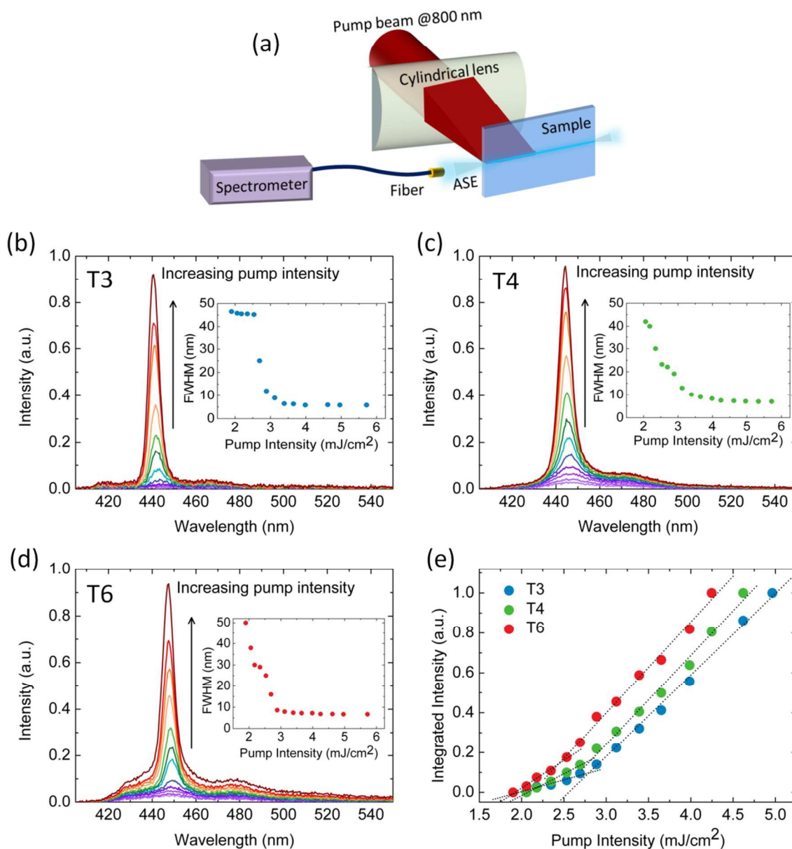
Figure 3. 2PA pumped ASE in the star-shaped oligomers with different arm-length. (a) Schematic of the experimental setup for the measurement of the ASE in the spin-coated samples of the oligomers. Two-photon pumped emission and ASE spectra in (b) T3, (c) T4 and (d) T6 molecules as a function of the increasing pump intensity. (b)-(d) The insets show the change of the FWHM emission as a function of the pump intensity. (e) Pump intensity vs integrated emission intensity in T3, T4 and T6 molecules under 2PA pumping clearly exhibiting a threshold behavior.
