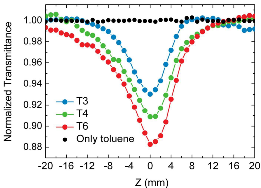
Figure 2. Open aperture z-scan measurement of the nonlinear absorption cross-section. Normalized transmittance of the Gaussian laser beam (800 nm, 120 fs and 1kHz repetition rate) through a 1 mm quartz cuvette containing 10 mM of T3, T4, T6 and only toluene, measured by the open aperture z-scan technique.
