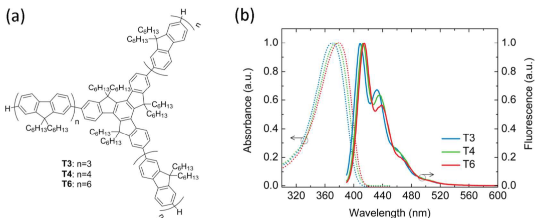
Figure 1. Molecular structure, emission and absorbance spectra of the star-shaped oligomers with different arm-lengths. (a) Molecular structure of the star-shaped truxene based oligofluorenes having varying fluorene arm length. (b) Solution-state absorbance and photoluminescence spectra of the T3, T4 and T6 star-shaped oligofluorenes.
