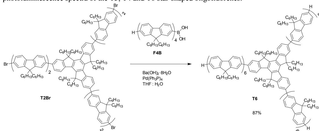
Scheme 1. Synthetic procedure for the T6 compound.
