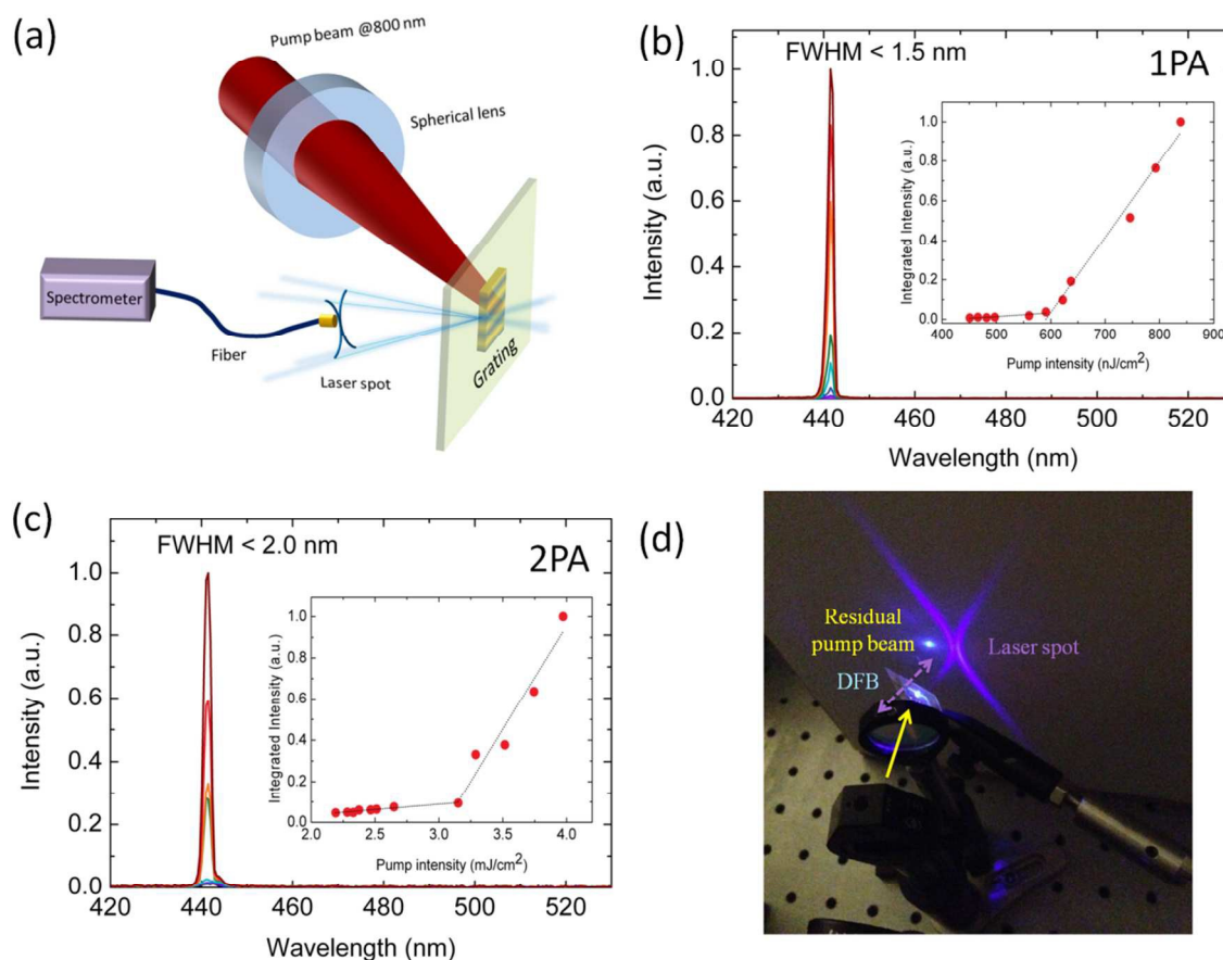
Figure 4. 1PA and 2PA pumped laser of the T6 molecules. (a) Schematic of the experimental setup for the characterization of the frequency up-converted laser of the T6 oligomer. Flexible DFB laser of T6 oligomer under (b) 1PA pumping and (c) 2PA pumping. (b)-(c) The insets show the pump intensity vs integrated emission intensity from the laser exhibiting the lasing thresholds. (d) Photograph of the frequency up-converted laser of T6 showing the fan-shaped laser beam on the screen.
