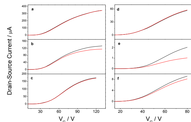
Fig. 3 Examples of I_D vs. V_G sweeps before (black) and after (red) switching from the open to the closed form by irradiation at 320 nm for (a) pristine PCBM, (b) PCBM/DAE-FN blend, (c) PCBM/DAE-F blend, (d) pristine ICBA, (e) ICBA/DAE-FN blend, and (f) ICBA/DAE-F blend.
