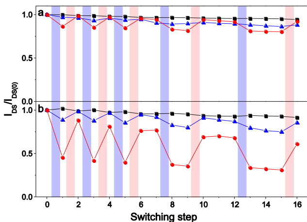
Fig. 4 Normalized drain-source current as a function of repeatedly switching the DAEs between their open and closed states for a) PCBM, and b) ICBA devices (black squares=pristine material, red circles=DAE-FN blend, and blue triangles=DAE-F blend). Lines are drawn as guide for the eye. Irradiation is indicated by violet ( \lambda = 320 nm, 30 s) and red ( \lambda = 540 nm, 10 min) shaded areas. For details regarding the switching procedure see the SI.
