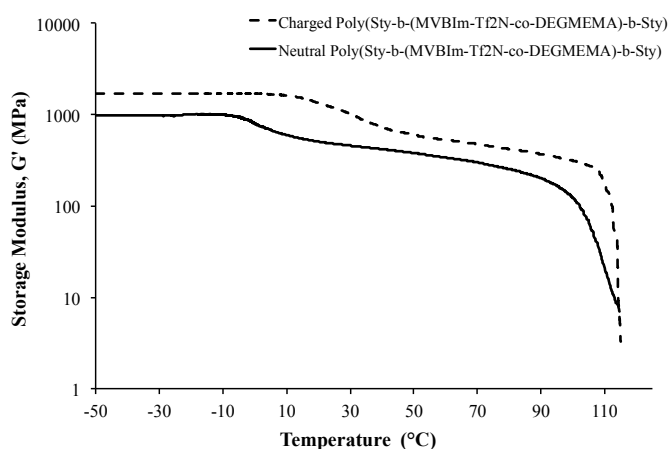
Figure 2: Dynamic mechanical analysis (DMA) of neutral and ionomeric A-BC-A triblock copolymer poly[Sty- b -(MVBIm-Tf 2 N-co-DEGMEMA) 48 ]- b -Sty].
