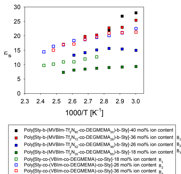
Figure 9. Temperature-dependence of static dielectric constant for A-BC-A triblock copolymers and random copolymers (open symbols).
