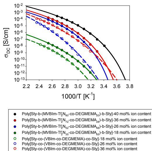
Figure 5: Temperature dependence of ionic conductivity which increases with increase in ion content and found to be more than random copolymers (open symbols).
