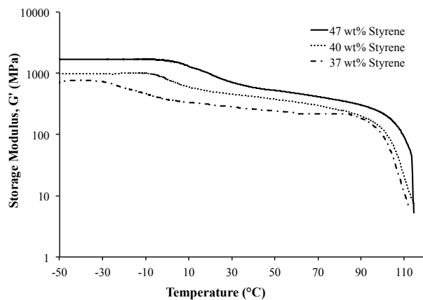
Figure 1: Dynamic mechanical analysis (DMA) of ionic A-BC-A triblock copolymer poly[Sty- b -(MVBIm-Tf 2 N- co -DEGMEMA)- b -Sty] with varying compositions.
