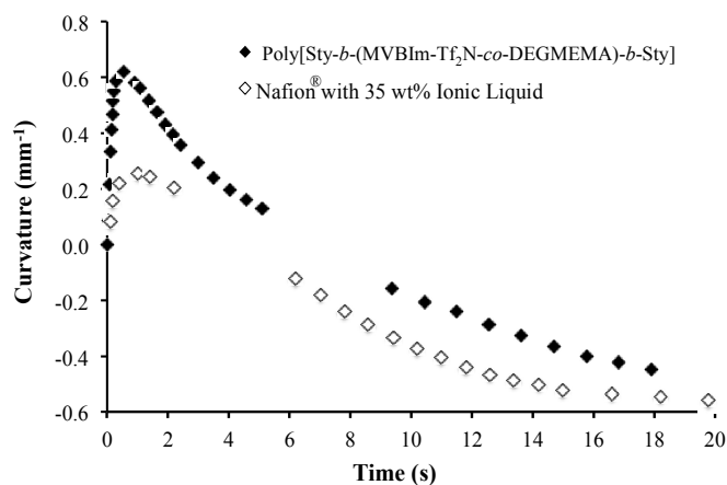
Figure 10: Curvature observed for electromechanical actuators made from poly[Sty- b -(MVBIm-Tf 2 N 52 - co -DEGMEMA 48 )- b -Sty] having 26 mol% ion content at ambient conditions (20 °C and ~ 43% RH) under a 4 V applied voltage after soaking the film in ionic liquid [EMIm][TfO], uptaking 30 wt%. The open symbols are for similar actuators that use Nafion with an uptake of 35 wt%.
