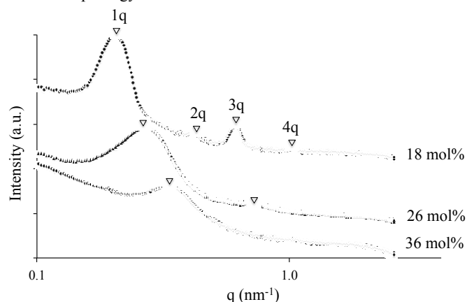
Figure 4: Small angle X-ray scattering (SAXS) of ionomeric A-BC-A triblock copolymer poly[Sty- b -(MVBIm-Tf 2 N-co-DEGMEMA)- b -Sty] with various ion contents 18, 26 and 36 mol%.
