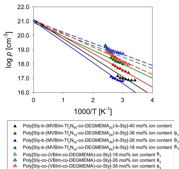
Figure 7: Temperature dependence of conducting ion concentration for A-BC-A triblock copolymers and random copolymers (open symbols) determined using the EP model.
