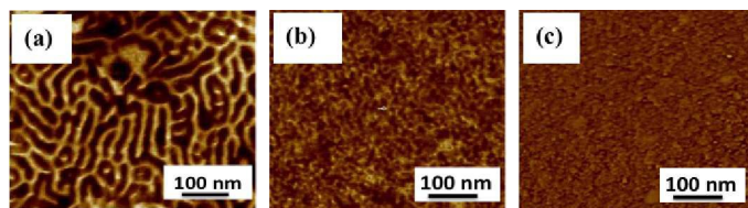
Figure 3: Atomic force microscopy (AFM) of ionomeric A-BC-A triblock copolymer poly[Sty- b -(MVBIm-Tf 2 N-co-DEGMEMA)- b -Sty] going from (a) 18 mol% (b) 26 mol% (c) 36 mol% ion content.
