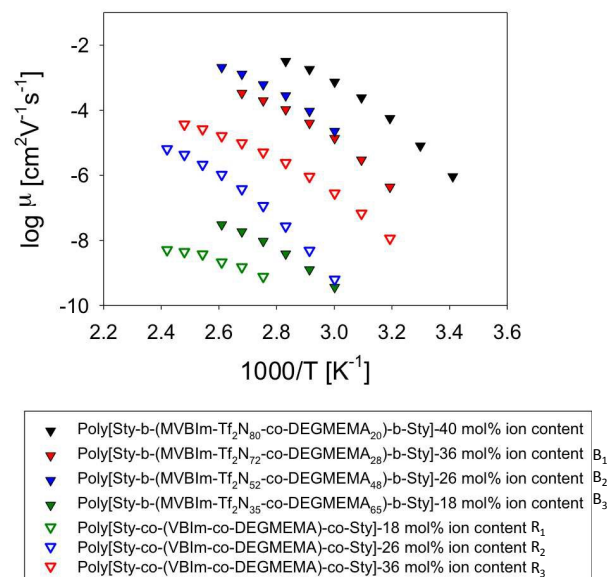
Figure 8. Temperature-dependence of ion mobility for A-BC-A triblock copolymers and random copolymers (open symbols) determined using the EP model
