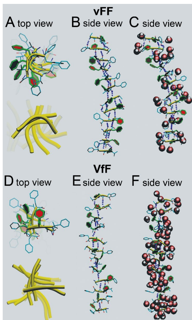
Fig. 7. Molecular modelling of dodecamer stacks of gelling tripeptides vFF (A-C) and Vff (D-F). Peptide backbones are highlighted in yellow, hydrogen bonds in blue, central phenylalanines in color, and water molecules are depicted as red spheres (C, F).
