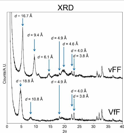
Fig. 6. XRD analysis of vFF and Vff hydrogels.
