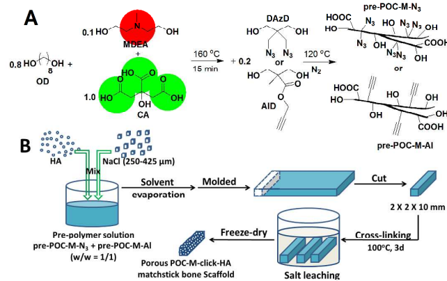
Figure 1. (A) Synthesis of N-methyl-diethanolamine (MDEA) modified poly(1,8-octanediol citrate)-click (POC-M-click) pre-polymers: pre-POC-M-N 3 and pre-POC-M-Al. (B) Fabrication process of POC-M-click-HA matchstick bone scaffold.
