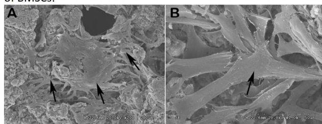
Figure 4. Scanning electron microscopy (SEM) images of bone marrow-derived mesenchymal stem cells (BMSCs) grown on the POC-M-click-HA scaffolds (3 days) taken at different magnifications: (A) 200× and (B) 1000×.
