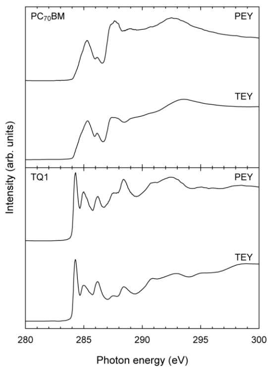
Figure 2. C1s NEXAFS spectra measured in total electron yield (TEY) and partial electron yield (PEY) of pristine PC 70 BM and pristine TQ1 films.
