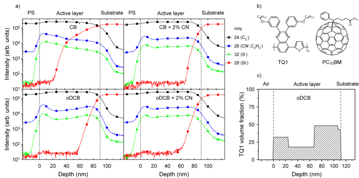
Figure 1. a) d-SIMS depth profiles for TQ1:PC 70 BM 1:3 w/w films spincoated on silicon substrates from CB, CB + 2% CN, oDCB and oDCB + 2% CN. PS refers to the polystyrene sacrificial layer. The vertical dashed lines mark the top and bottom of the active layer; the top of the active layer is drawn where the intensity of the S - signal (green) has reached 50% of the maximum intensity value of the first peak whereas the bottom of the active layer is drawn where the C 2 - signal has dropped to 50% of its saturation intensity inside the active layer. For more details on the interpretation of the m/q = 26 signal, see the supplementary information. b) Molecular structures of TQ1 and PC 70 BM. c) Ellipsometrically deduced polymer volumetric depth profile for a TQ1:PC 70 BM 1:3 w/w film spincoated from oDCB onto silicon.
