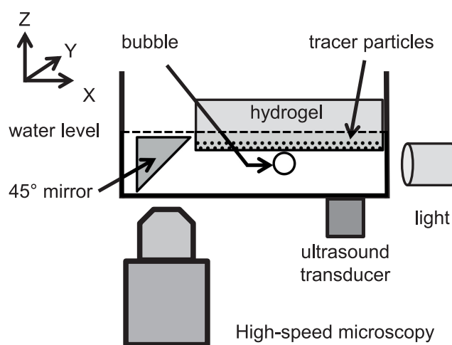
Fig. 1 Schematic diagram of the experimental setup and definition of coordinate system. The surface of the gel lies in the (x,y) plane. The vertical axis z points into the gel layer.
