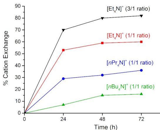
Fig. 2 Cation exchange (%) of [R 4 N] + by [Cp 2 Co] + determined by ICP-OES for [(Cp 2 Co) x (R 4 N) 3-x ][In 3 (BTC) 4 ] (x = 3 corresponds to 100%). Conditions: 0.02 M solution of [Cp 2 Co][PF 6 ] in acetone, initial ratio [R 4 N] + /[Cp 2 Co] + = 1/1 or 3/1.
