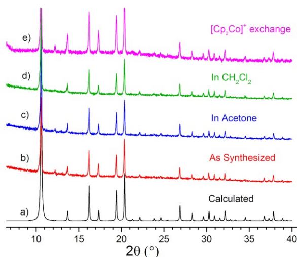
Fig. 1 Comparison of Powder X-ray Diffraction (PXRD) patterns of [TEA] 3 [In 3 (BTC) 4 ]: (a) calculated from the single crystal structure, (b) as synthesized, (c) after soaking for one day at 298 K in acetone or (d) CH 2 Cl 2 and (e) after [Cp 2 Co] + exchange in acetone.
