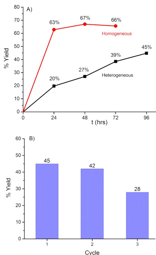
Fig. 8 A) Yield vs time plot of heterogeneous (black) and homogeneous (red) DA reaction under identical conditions (10 mol% [Fe]/[MVK] in CH 2 Cl 2 , [Iso] = 0.4 M, [MVK] = 0.1 M). B) Recycling of [(Fp-L) 0.6 (TEA) 2.4 ][In 3 (BTC) 4 ] under the same conditions. Each cycle lasts 96 h.
