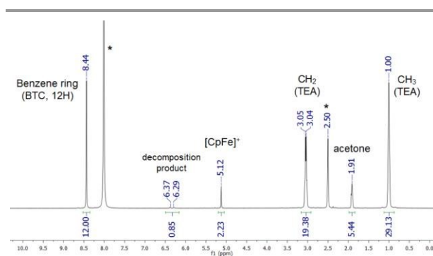
Fig. 7 ^1\text{H} NMR spectrum of [(\text{Fp-L})_{0.6}(\text{TEA})_{2.4}][\text{In}_3(\text{BTC})_4] after digestion in \text{DCI}/d^6\text{-dmsO} (1/5 v/v). NMR solvent peaks are marked with an asterisk.
