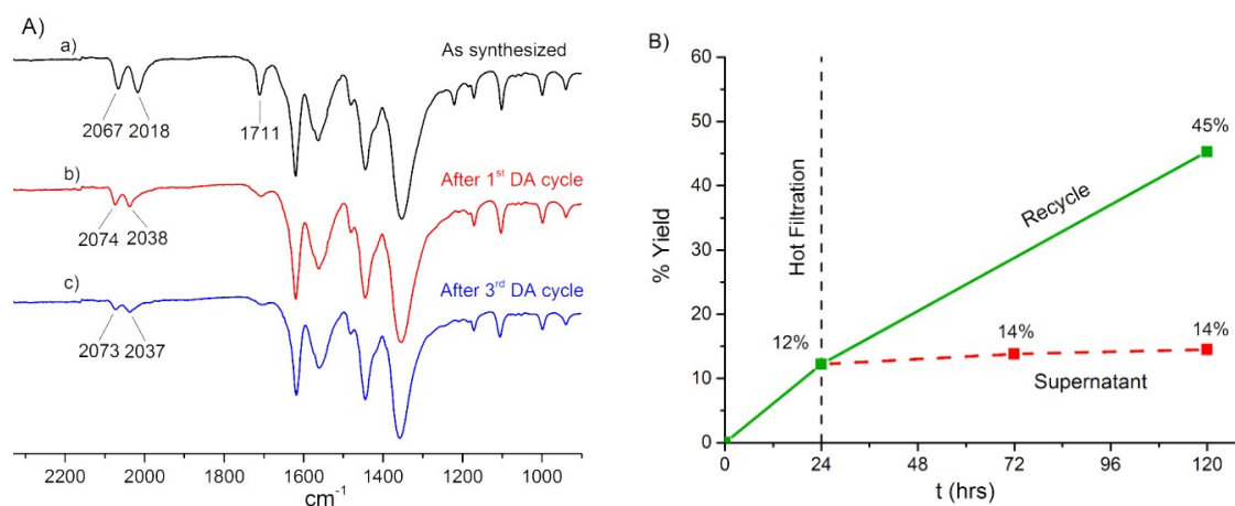
Fig. 9 A) IR spectrum of [(Fp-L)_{0.6}(TEA)_{2.4}][In_3(BTC)_4] (a) as synthesized, (b) after one and (c) after three catalytic cycles. Each cycle lasts 96 h. Spectra have been normalized to the highest intensity peak for the sake of comparison. B) Leaching test for [(Fp-L)_{0.6}(TEA)_{2.4}][In_3(BTC)_4] . The DA reaction essentially stops in the supernatant after filtering off the catalyst (red dashed line). The solid catalyst is still active if a fresh batch of reactants is added (green solid line).
