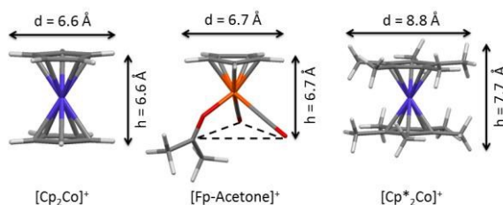
Fig. 3 Dimensions of organometallic cations tested for cation exchange (corrected for Van der Waals radii). 85-86 [Fp-acetone] + was modelled by truncating the tropone ligand in the single-crystal structure of [Fp-tropone][BF 4 ]. 103
