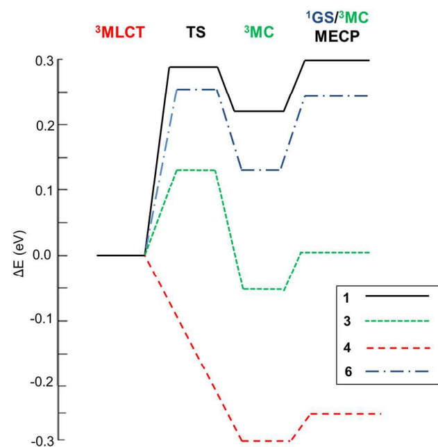
Figure 1. Relative energetic profile (B3LYP/6-31G(d)) of the temperature-dependent non-radiative pathways of 1, 3, 4 and 6. The reference is the 3 MLCT emissive state.
