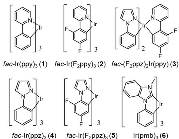
Chart 1. Chemical structure of complexes 1-6.
