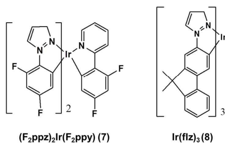
Chart 2. Chemical structure of the validator complexes 7-8.
