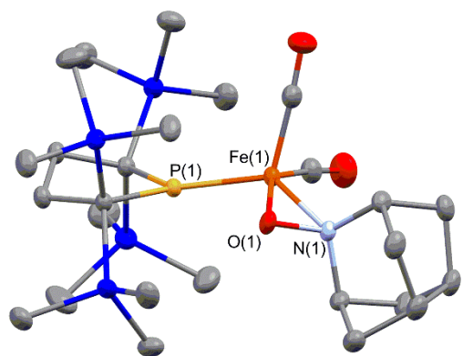
Figure 7. Molecular structure of 4 with 50 % probability ellipsoids.
