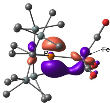
Figure 6. Graphical representations of the DFT(PBE0)-derived \beta HOMO for 3 opt .
