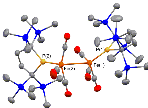
Figure 1. Molecular structure of 2 with 50 % probability ellipsoids.
