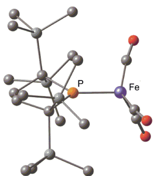
Figure 5. DFT(PBE0) optimized structure of 3 opt .
