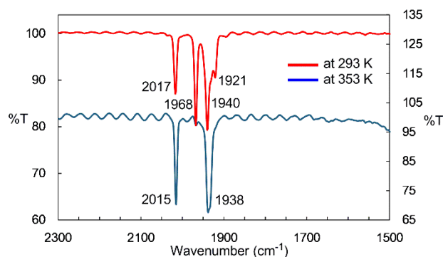
Figure 2. IR spectra of the n -octane solution of 2 at 293 K and 353 K.
