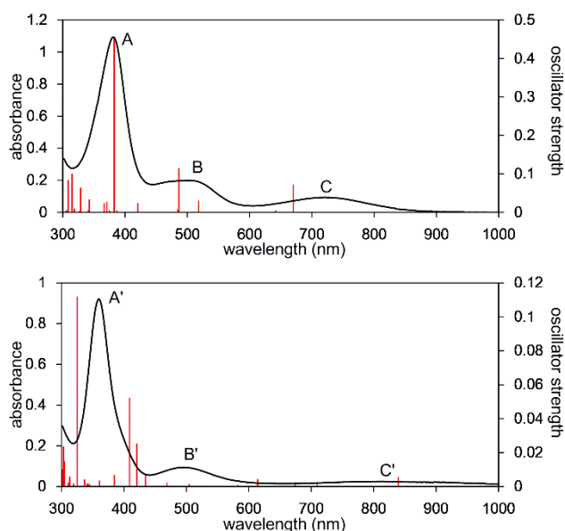
Figure 3. UV-vis-NIR spectra of the n -octane solution of 2 measured at 293 K (upper) and 353 K (lower). Solid red bars indicate the calculated transition of the \mathbf{2}_{\text{opt}} (upper) and \mathbf{3}_{\text{opt}} (lower).
