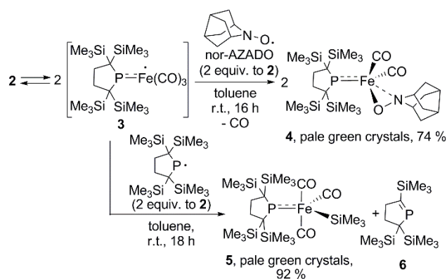
Scheme 3. Reactions of in situ generated 3 with organic radicals.
