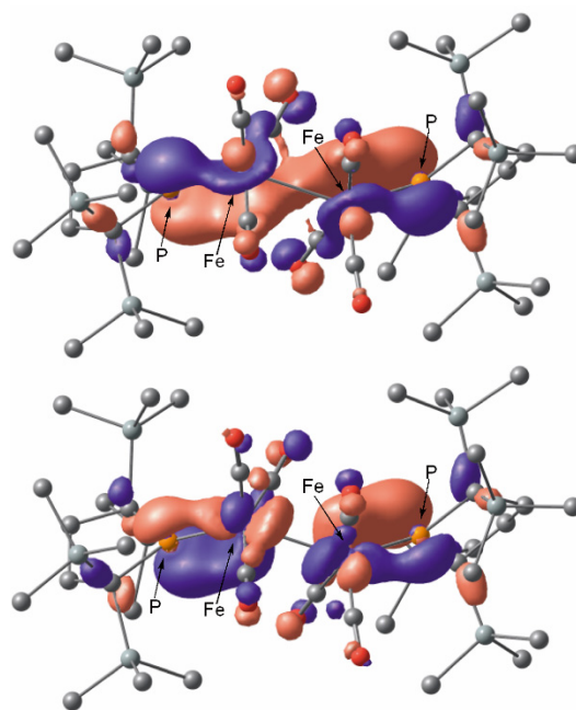
Figure 4. Graphical representations of the DFT(PBE0)-derived HOMO (upper) and HOMO-1 (lower) for \mathbf{2}_{\text{opt}} .
