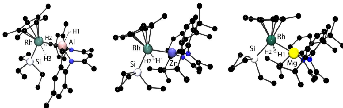
Figure 1. The crystal structures of 1 (left), 2 (middle) and 3 (right). Selected bond angles and bond lengths. 1 : Rh–Si 2.3402(8), Rh–Al 2.4527(8), Si–Rh–Al 102.82(3). 2 : Rh–Si 2.3571(8), Rh–Zn 2.4158(4), Si–Rh–Zn 106.86(2). 3 : Rh–Si 2.3437(7), Rh–Mg 2.5049(8), Si–Rh–Mg 106.23(2). Hydrides were located within the Fourier difference maps.
