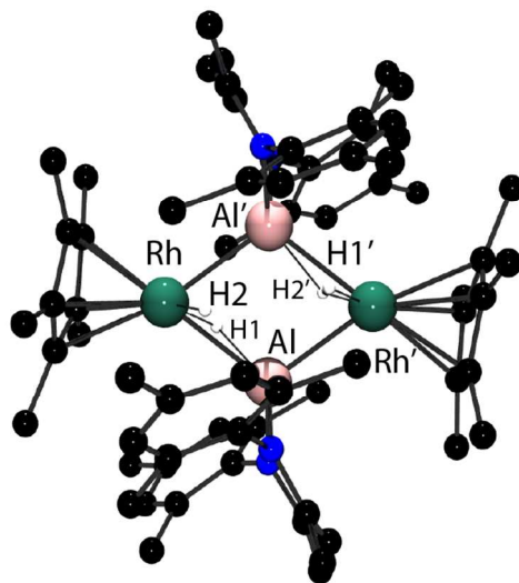
Figure 5. The crystal structure of 4 2 . Selected bond angles (°) and bond lengths (Å). Rh–Al 2.5282(7), Rh–Al' 2.4973(7), Al–Rh'–Al 70.97(2), Rh–Al–Rh' 108.94(2). Hydrides were located within the Fourier difference map.
