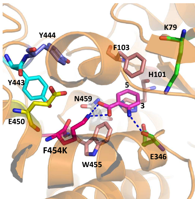
Figure 4. X-ray crystal structure of PrnA F454K mutant (PDB 4Z44) with anthranilic acid ( 4 ) positioned in the active site showing possible H-bonding interactions with the substrate.
