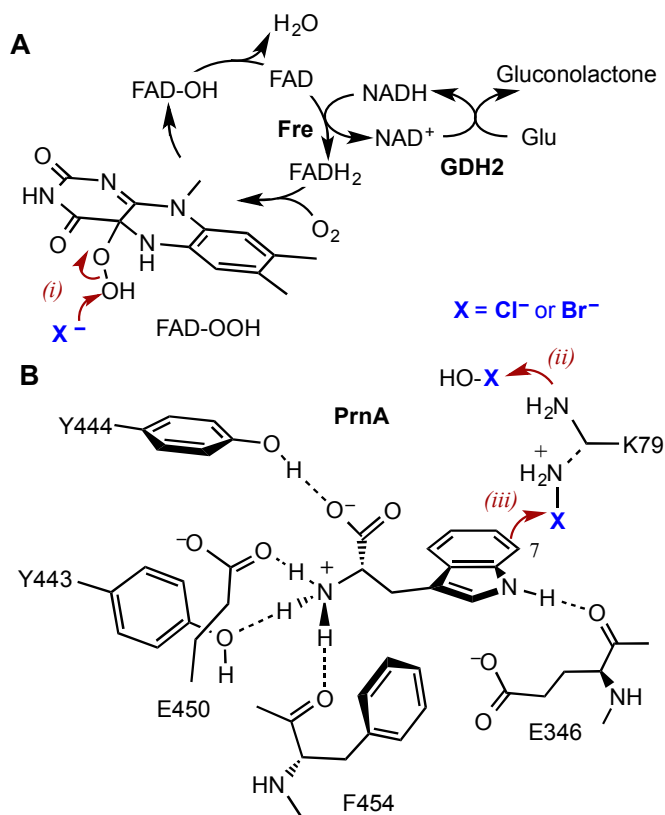
Figure 1. The mechanism of the tryptophan 7-halogenase PrnA. (A) The flavin reductase from Escherichia coli (Fre) and glucose dehydrogenase (GDH2) from Bacillus megaterium were used to recycle FAD and NAD + . (B) PrnA active site with the tryptophan substrate bound. Residues which stack above and below the substrate indole are removed for clarity. The hypohalous acid generated (step i), reacts with the amino group of K79 (step ii) resulting in a chloroamine electrophile which attacks the indole C7 (step iii). E346 acts as a general base to deprotonate the \sigma -complex.
