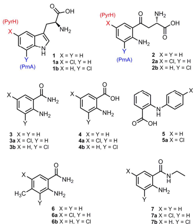
Figure 2. Substrates and products from reactions with PyrH and PrnA.
