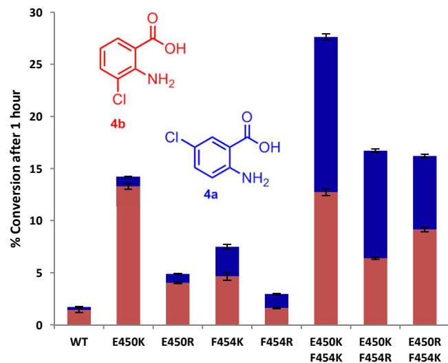
Figure 3. The % chlorination of anthranilic 4 , by PrnA mutants, and ratios of products 5- and 3-chloroanthranilic acid ( 4a & 4b ) after 1 hour with halogenase enzyme (10 \mu M) and substrate (0.5 mM).
