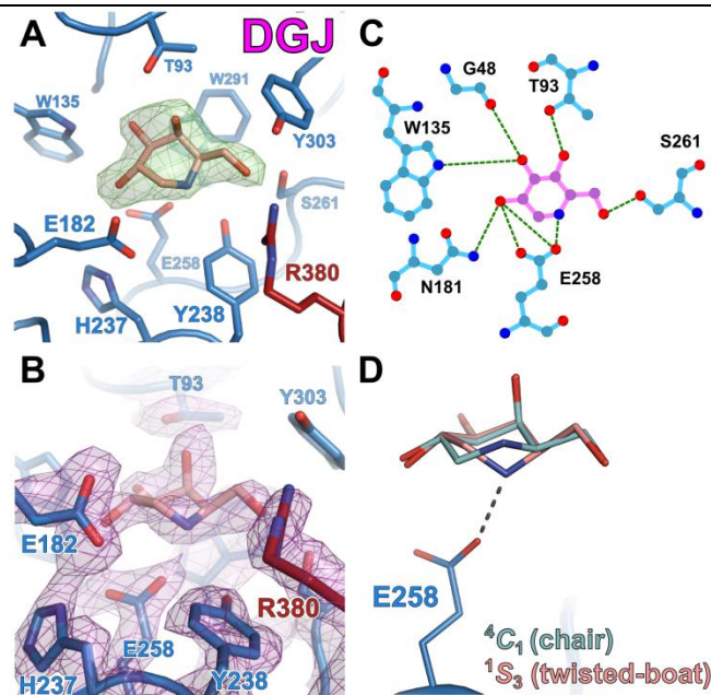
Fig. 6. DGJ binds the active site in a distorted {}^1S_3 conformation. (A) Unbiased difference electron density map ( F_o - F_c , 3.0 \sigma , green) before DGJ ligand refinement. (B) GALC active site with bound ligand, showing active site residues (sticks) and refined, feature-enhanced electron density map ( 0.65 e^{-}/\text{\AA}^3 , purple). (C) Schematic representation of hydrogen bond interactions (green lines) between GALC and DGJ. (D) Adoption of the {}^1S_3 twisted-boat conformation allows DGJ to form a hydrogen bond with the nucleophile E258.
