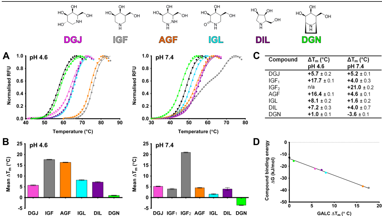
Fig. 4. Stabilization of GALC by azasugar compounds (A) Chemical diagrams of the molecules used in melt curves of GALC alone (black) and with 5.0 mM compound (colored, as above). Experiments were performed in sodium acetate, pH 4.6 and PBS, pH 7.4. (B) Bar graph showing the mean \Delta T_m \pm \text{SEM} conferred by 5.0 mM compound at pH 4.6 and pH 7.4. Experiments were performed in triplicate. (C) Values for mean \Delta T_m \pm \text{SEM} are tabulated. (D) Relationship between free energy of compound binding ( \Delta G ) and GALC stabilization \Delta T_m at pH 4.6. \Delta G values for each compound were calculated from the measured K_i (Fig. 3) using the equation \Delta G = RT \ln Ki , where R is the gas constant (8.31 J K -1 mol -1 ) and T is absolute temperature (310 K).
