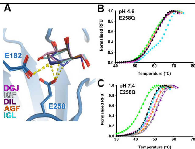
Fig. 8. Azasugar interaction with E258 is essential for optimal GALC stabilization. (A) Alignment of azasugar compounds bound in the GALC active site. Refined structures are overlaid, colored as indicated. Hydrogen bonds to catalytic residues E258 and E182 are shown (yellow lines). (B and C) Overlaid melt curves of GALC E258Q alone (black) and with 10 mM compound (colored as above). Experiments were performed in (B) sodium acetate, pH 4.6 and (C) PBS, pH 7.4.
