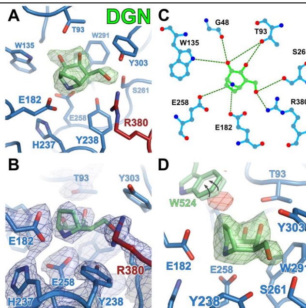
Fig. 7. DGN destabilizes GALC due to a steric clash in the active site. Unbiased difference electron density map ( F_o - F_c , 3.0 \sigma , green) before DGN ligand refinement. (B) GALC active site with bound ligand, showing active site residues (sticks) and refined 2mF_o - DF_c electron density map ( 0.25 \text{ e}/\text{\AA}^3 , blue). (C) Schematic representation of hydrogen bond interactions (green lines) between GALC and DGN. (D) Unbiased difference electron density ( F_o - F_c ; +3.0 \sigma green, -3.0 \sigma red) illustrating the steric clash between the ethylene bridge of DGN and W524 of the GALC lectin domain.
