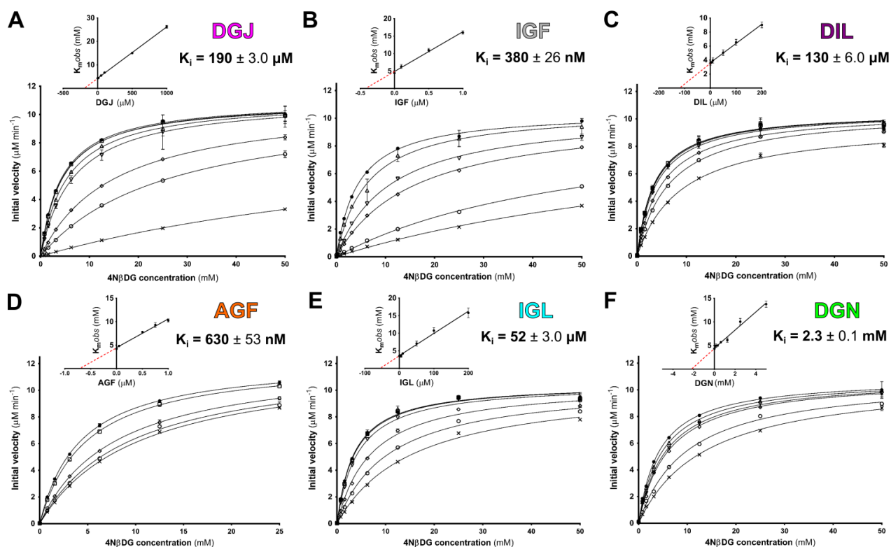
Fig. 3. Competitive inhibition kinetics of galacto -configured azasugars. Plots of GALC initial velocity vs. substrate concentration with (A) DGJ, (B) IGF, (C) DIL, (D) AGF, (E) IGL and (F) DGN at concentrations encompassing the K_i (see Supporting Methods). Inset Plots of K_{m,obs} vs concentration showing -K_i as the X-intercept. SEM error bars are shown.
