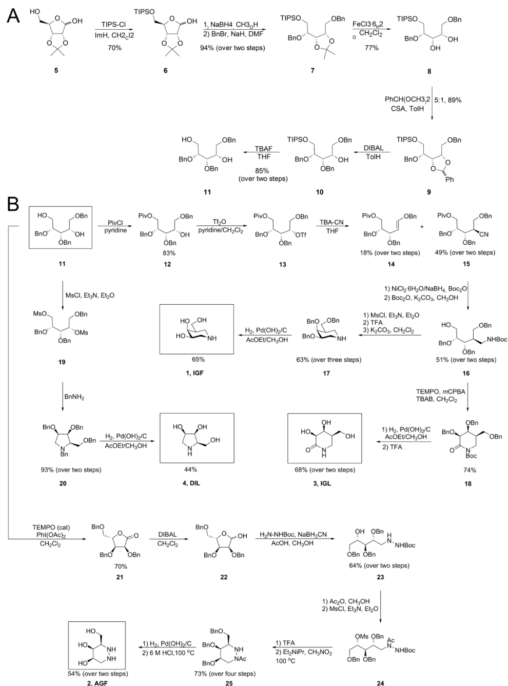
Fig. 2. Synthesis of azasugars. (A) Synthesis of key intermediate 11 from 2,3-O-isopropylidene-D-ribofuranose (5). (B) Synthesis of IGF, IGL, DIL and AGF from a common intermediate (11).
