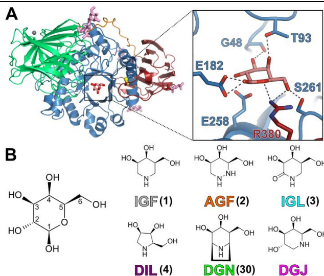
Fig. 1. Structure of GALC and azasugar compounds. (A) Ribbon diagram of GALC illustrating the \beta -sandwich (red), TIM-barrel (blue) and lectin (green) domains with \beta -D-galactose in the active site and N-linked glycans (pink sticks). Hydrogen bonding interactions (dashed lines) between galactose and active site residues are shown (zoomed box). (B) Pyranose ring numbering of \beta -D-galactose illustrating the anomeric position and chemical diagrams of the molecules used in this study: deoxy- galacto -nojirimycin (DGJ); iso- galacto -fagomine (IGF); dideoxyiminolixitol (DIL); iso- galacto -fagomine lactam (IGL); aza- galacto -fagomine (AGF) and deoxy- galacto -noeurostegine (DGN). Compounds are color coded as indicated throughout this study.
