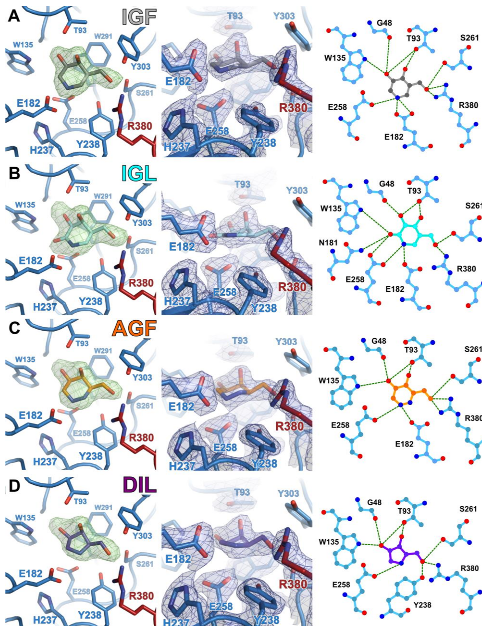
Fig. 5. Structures of chaperone molecules bound in the GALC active site. X-ray crystal structures of (A) IGF, (B) IGL, (C) AGF and (D) DIL bound in the GALC active site. Compounds are colored as indicated. ( Left panel ) Unbiased difference electron density maps ( F_0 - F_C , 3.0 \sigma , green) before ligand modelling at the active site of GALC. ( Centre panel ) Detail of the GALC active site with bound ligand, showing active site residues (sticks) and refined 2mF_0 - DF_C electron density contoured at 0.25 e^-/\text{\AA}^3 (blue). ( Right panel ) Schematic representation of hydrogen bond interactions (green dashed lines) between GALC and ligands.
