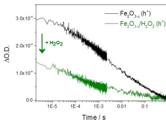
Fig. 5 TA decay traces recorded at 700 nm of photoholes on \alpha\text{-Fe}_2\text{O}_{3-x} at 1.4 V_{\text{RHE}} in 1 \text{ M NaOH} in the absence and presence of a hole scavenger ( 0.5 \text{ M H}_2\text{O}_2 ).
