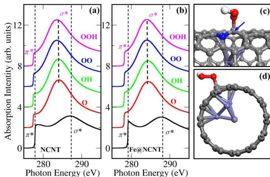
Fig. 5 Calculated X-ray absorption spectra at K-edge of carbon in the vicinity of encapsulated Fe_4 cluster for a bare SWCNT (black curves) and for the same SWCNT with adsorbed oxygen-containing species (color curves). (a) NCNT, (b) Fe@NCNT, (c) top and
