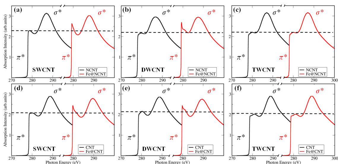
Fig. 3 Calculated X-ray absorption spectra of carbon atoms at K-edge on CNTs with and without \text{Fe}_4 cluster (see Fig. S8 in Supplementary Information for calculation details and models). (a) A single-walled CNT (SWCNT), (b) a double-walled CNT (DWCNT), and (c) a triple-walled CNT (TWCNT) with a nitrogen dopant in the vicinity of the probed carbon atom; and undoped (d) SWCNT, (e) DWCNT, and, (f) TWCNT, respectively.
