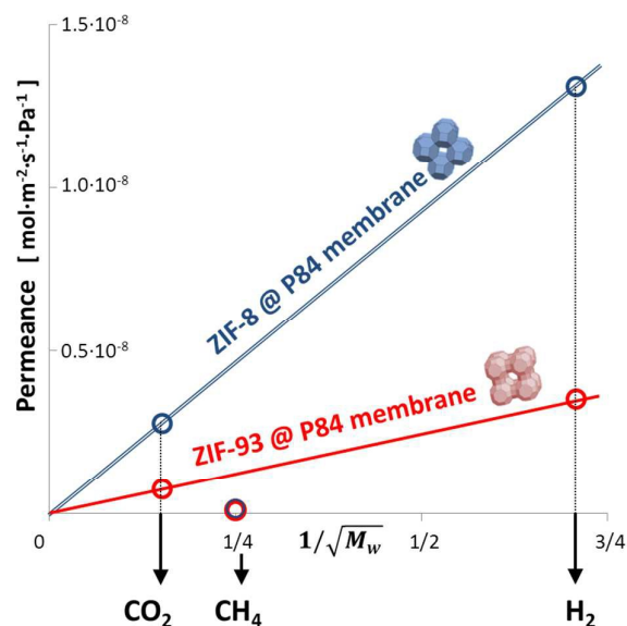
Figure 7. Gas permeances of the in situ annealed ZIF-8@P84 and ZIF-93@P84 HF membranes at 35 °C with respect to the inverse of the square root of the molecular weight of the gas molecule.
