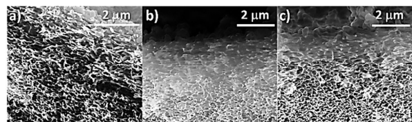
Figure 5. SEM cross-section images of the raw P84 HF polymer (A-type), the vacuum (C-type) and in situ (B-type) annealed P84 HFs, showing some densification and decreasing of the free volume near the surface.
