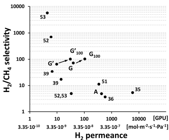
Figure 8. H 2 /CH 4 performance comparison of the ZIF-8@P84 and ZIF-93@P84 HF membranes (measured at 35 and 100 °C, see Figures 2 and S3) with the performances of previously reported HF membranes: those of MOFs, 35,36,39 pure polyimide 51-53 and some CMSMs 52,53 derived from them. See supplementary data for additional information in Table S3. All data were obtained in the 20-60 °C temperature range with the exception of G 100 and G' 100 .
