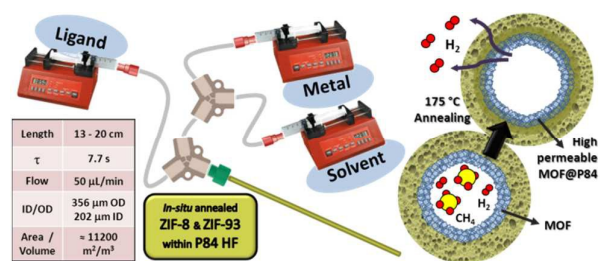
Figure 1. Experimental microfluidic setup for the fabrication of ZIF-93 and ZIF-8 membranes, including some working parameters and their diagrammatic application in gas separation.
