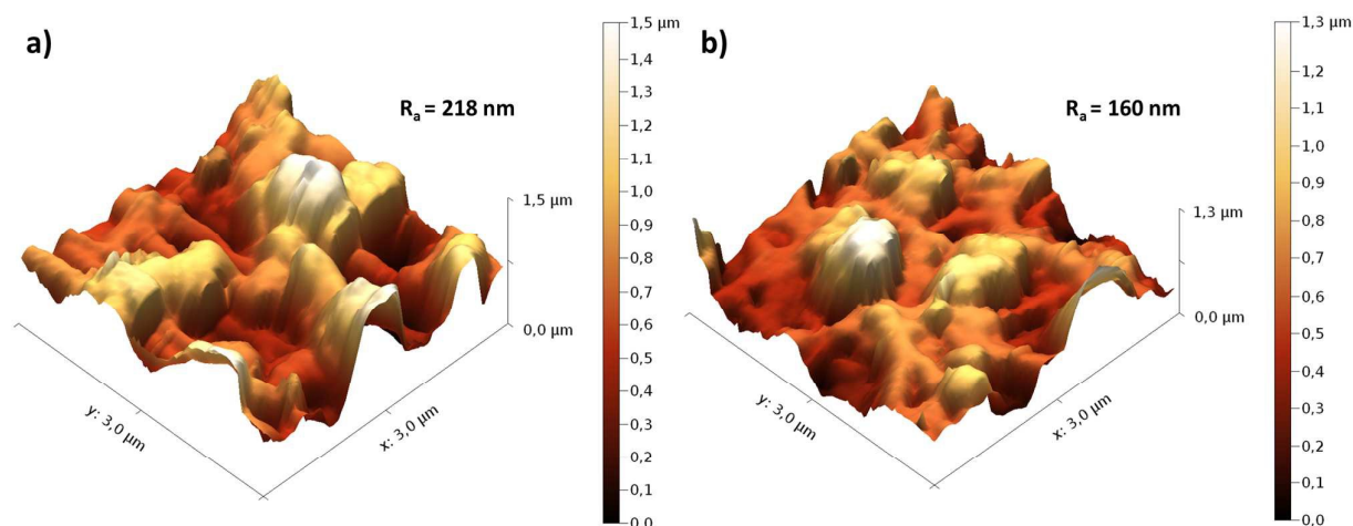
Figure 6. AFM 3D surface rendering and averaged surface roughness ( R_a ) of the inner side of a raw (a) and a vacuum annealed (b) selected areas of the P84 hollow fiber supports.
