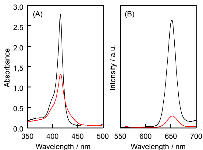
Fig. 3 (a) UV-vis absorption spectra of the 1•TMe-β-CDx complex (black line) and LMI1 (red line) and (b) the fluorescence spectra of the 1•TMe-β-CDx complex (black line) and LMI1 (red line).
