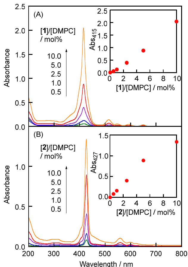
Fig. 2 UV-vis absorption spectra of (a) LMI1 and (b) LMI2 prepared by the exchange method at 30 °C for 1 h ([DMPC] = 1.0 mM, [1] or [2]/[DMPC] = 0.5, 1.0, 2.5, 5, and 10.0 mol%). Inset: the absorbance (Abs) at \lambda_{\max} versus [1]/[DMPC] in LMI1 or [2]/[DMPC] in LMI2 prepared by the exchange method.
