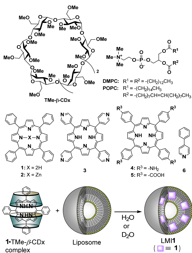
Scheme 1. Structures of compounds and exchange reaction of 1.
