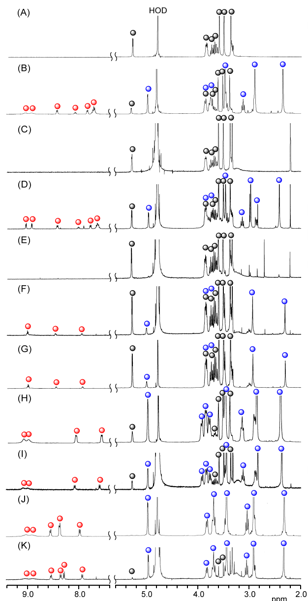
Fig. 4 Partial ^1\text{H} NMR spectra of (A) TMe- \beta -CDx, (B) the 1•TMe-β-CDx complex, (C) a mixture of the 1•TMe-β-CDx complex and the DMPC liposomes, (D) the 2•TMe-β-CDx complex, (E) a mixture of the 2•TMe-β-CDx complex and the DMPC liposomes, (F) the 3•TMe-β-CDx complex, (G) a mixture of the 3•TMe-β-CDx complex and the DMPC liposomes, (H) the 4•TMe-β-CDx complex, (I) a mixture of the 4•TMe-β-CDx complex and the DMPC liposomes (J) the 5•TMe-β-CDx complex and (K) a mixture of the 5•TMe-β-CDx complex and the DMPC liposomes ([1, 2, 3, 4 or 5]/[DMPC] = 10.0 mol%) in \text{D}_2\text{O} at 25 °C (•: free TMe- \beta -CDx, •: 1, 2, 3, 4 or 5 and •: TMe- \beta -CDx in the 1, 2, 3, 4 or 5•TMe-β-CDx complex)
