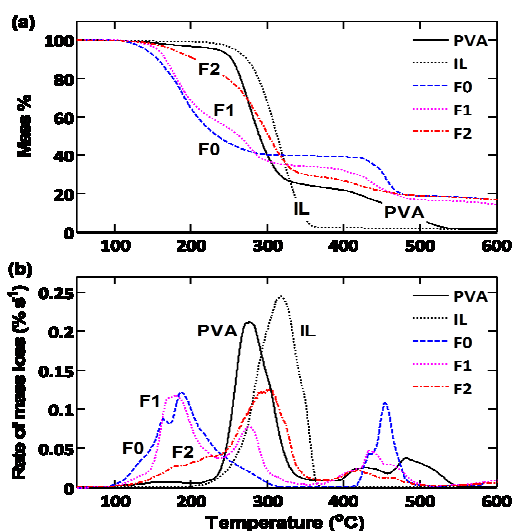
Fig. 1 (a) TG and (b) DTG plots of PVA, IL and precursor films F0, F1 and F2; 10 °C min -1 heating rate and 20 cm 3 min -1 N 2 purge.
