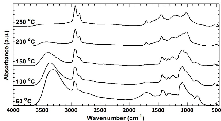
Fig. 2 FTIR spectra of PVA precursor film, F0, heated in vacuum for 1 h at different temperatures.
