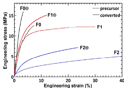
Fig. 8 Stress vs. strain data for the precursor and converted films (⊕) acquired at 35 °C in the tensile mode. Precursor film F2 showed strain of about 106 % before failure, but the scale of the strain axis is truncated for clarity.
