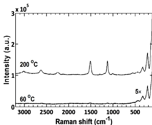
Fig. 4 Raman spectra of film F2, before and after heating in vacuum at 200 °C for 1 h; spectra acquired using 514.5 nm excitation wavelength.
