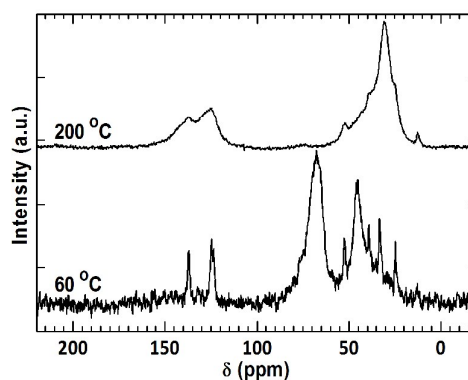
Fig. 3 13 C NMR spectra of film F2, before and after heating in vacuum at 200 °C for 1 h.
