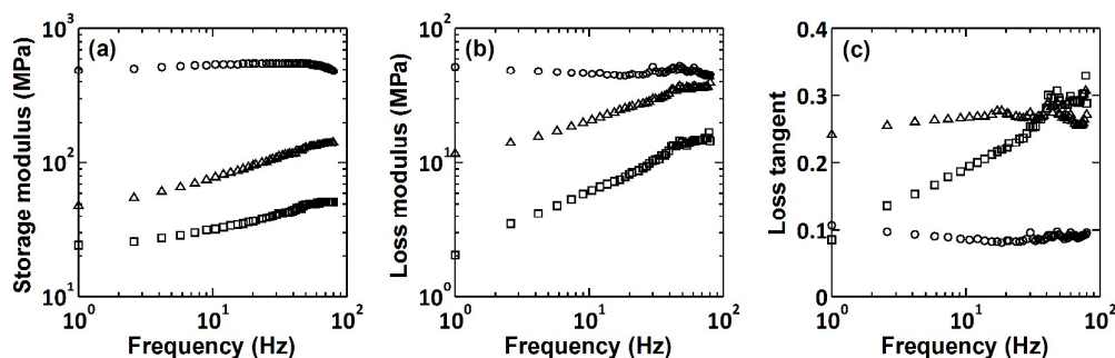
Fig. 7 DMA results of fully-dehydrated films, F0 (○), F1 (Δ), and F2 (□), at 115 °C: (a) storage modulus, (b) loss modulus, and (c) loss tangent; 1 % oscillation amplitude and nitrogen atmosphere.
