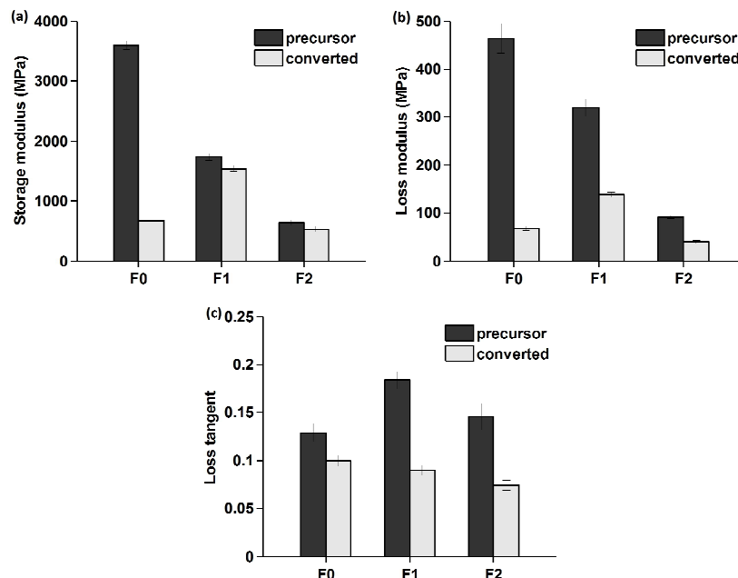
Fig. 6 DMA results of the precursor and converted films, F0, F1, and F2, at 35 °C: (a) storage modulus, (b) loss modulus, and (c) loss tangent; 1 % oscillation amplitude, 1 to 80 Hz frequency, and nitrogen atmosphere.
