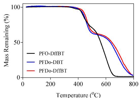
Figure 4. TGA plots of PFO-DffBT , PFDo-DBT , and PFDo-DffBT with a heating rate of 10°C min -1 under an inert atmosphere of nitrogen.
