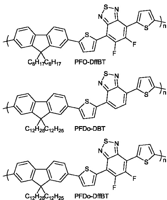
Figure 1. Structures of PFO-DffBT , PFDo-DBT and PFDo-DffBT .
