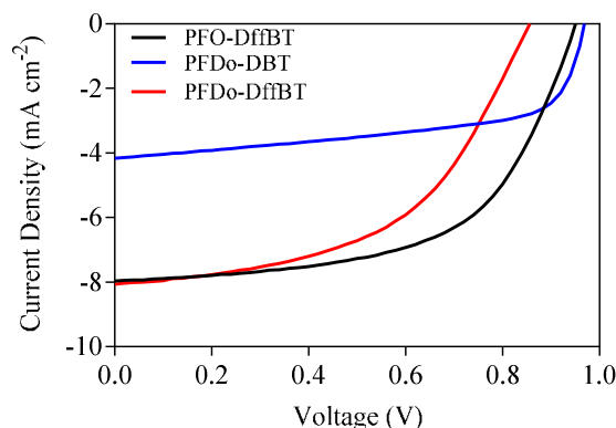
Figure 6. J-V characteristic curves of photovoltaic devices fabricated from PFO-DffBT , PFDo-DBT and PFDo-DffBT .
