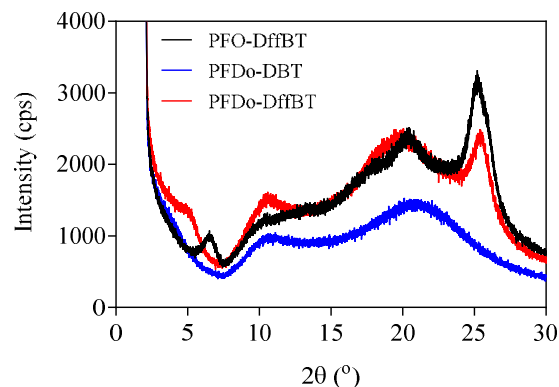
Figure 5. Powder X-ray diffraction (XRD) patterns of PFO-DffBT , PFDo-DBT and PFDo-DffBT .
