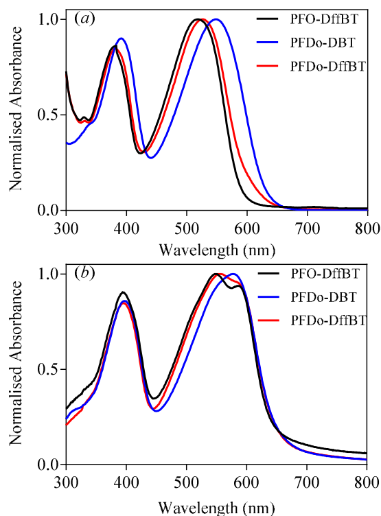
Figure 2. Normalised absorption spectra of PFO-DffBT , PFD o -DBT and PFD o -DffBT in; (a) chloroform solutions; and (b) thin films.
