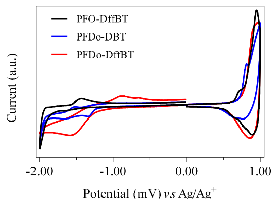
Figure 3. Cyclic voltammograms of PFO-DffBT , PFDo-DBT and PFDo-DffBT on platinum disc electrodes (area 0.031 cm 2 ) at a scan rate of 100 mV s -1 in acetonitrile/tetrabutyl ammonium perchlorate (0.1 mol dm -3 )
