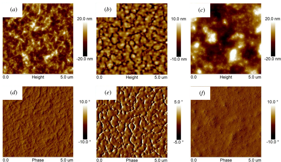
Figure 7. Tapping-mode atomic force microscopy topography ( a, b, c ) and phase images ( d, e, f ) of; PFO-DffBT:PC 70 BM (1:4 w/w, 3% DIO) ( a, d ); PFDo-DBT:PC 70 BM (1:4 w/w) ( b, e ); and PFDo-DffBT:PC 70 BM (1:4 w/w, 3% DIO) ( c, f ).
