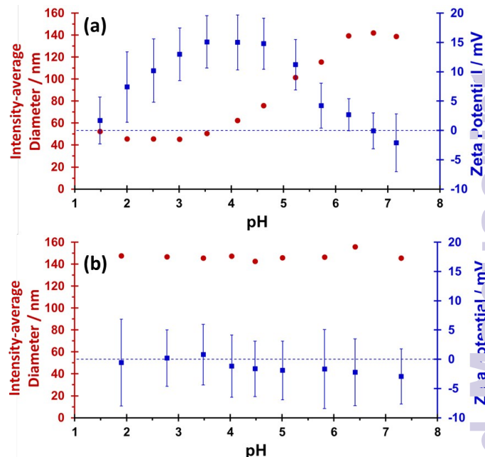
Figure 3 Hydrodynamic diameter vs. pH and zeta potential vs. pH curves obtained for (a) MPETTC-PGMA 50 -PHPMA 140 and (b) MePETTC-PGMA 58 -PHPMA 160 diblock copolymer nano-objects synthesised by RAFT aqueous dispersion polymerisation of HPMA at pH 7.0-7.5. Measurements are reported for 0.1% w/w copolymer dispersions prepared in the presence of 1 mM KCl. All pH titrations were performed from high pH to low pH. Error bars for zeta potential data are equivalent to 1 standard deviation.
