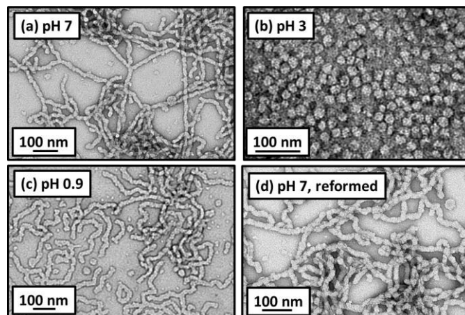
Figure 5 TEM images and corresponding digital photographs obtained for MPETTC-PGMA 50 -PPHMA 140 diblock copolymer nano-objects prepared via RAFT aqueous dispersion polymerisation of HPMA: (a) pH 7.2, (b) pH 3.0, (c) pH 0.9 and (d) after a pH switch from pH 7.2 to 3.0 to 7.3. A worm-to-sphere transition is observed on lowering the dispersion pH from 7.2 to 3.0. Further reduction in pH to 0.9 induces a sphere-to-worm transition, as excess acid acts as a salt.
