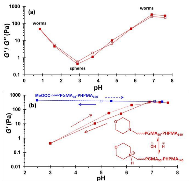
Figure 4. (a) Variation in G' (filled squares) and G'' (open squares) with respect to pH for MPETTC-PGMA 50 -PPHMA 140 diblock copolymer nano-objects at 15% w/w solids after switching from pH 7.6 to pH 0.9. (b) Variation in G' for the same MPETTC-PGMA 50 -PPHMA 140 diblock copolymer nano-objects on lowering the solution pH from pH 6.8 to pH 3.0 (solid red line) and returning from pH 3.0 to pH 7.3 (red dotted line). Similar pH switch experiments conducted on a control sample of MePETTC-PGMA 58 -PPHMA 160 diblock copolymer worms from pH 7.1 to pH 2.5 (blue solid line) and returning to pH 7.8 (blue dotted line). For the former worm gel, there is a reversible worm-to-sphere-worm transition mediated via protonation of the morpholine end-groups located on the PGMA stabiliser blocks. In contrast, no pH-responsive behaviour is observed for the latter worm gel, since these copolymer chains do not contain suitable end-groups.
