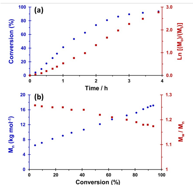
Figure 2 (a) Monomer conversion vs. time and (b) number-average molecular weight ( M_n ) and polydispersity ( M_w/M_n ) vs. conversion plots as determined by 1 H NMR and DMF GPC analyses, respectively, for the RAFT solution polymerisation of glycerol monomethacrylate in ethanol at 56 °C. Conditions: 45% w/w solids; target DP = 70; [MPETTC]/[AIBA] molar ratio = 5.0. M_w and M_n values were determined by DMF GPC calibrated with a series of ten near-monodisperse poly(methyl methacrylate) standards.
